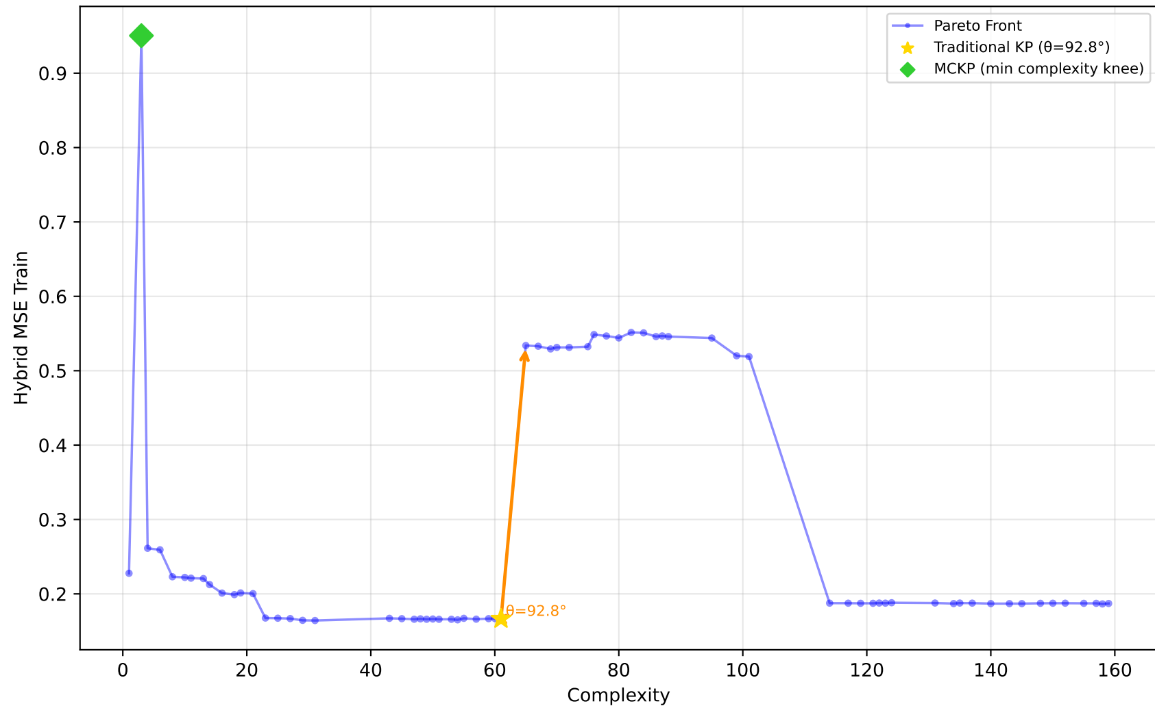
561_cpu - Run 9 - MVP - Hybrid MSE Train \lambda_1=0.70, \lambda_2=0.00, \lambda_3=0.10 | Difficulty: 0.55 | Method: mckp
