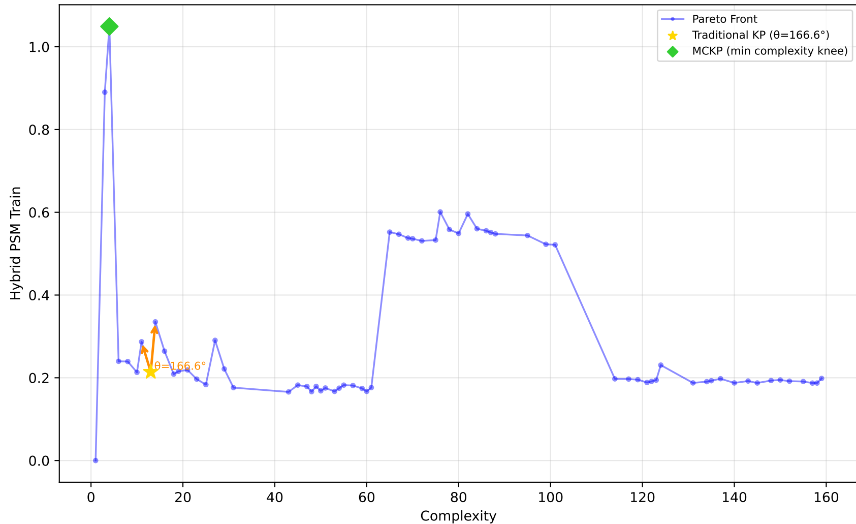
561_cpu - Run 9 - MVP - Hybrid PSM Train \lambda_1=0.70, \lambda_2=0.00, \lambda_3=0.10 | Difficulty: 0.55 | Method: mckp
