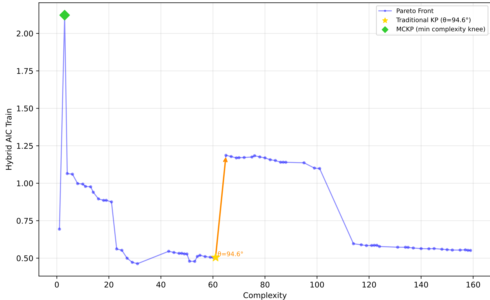
561_cpu - Run 9 - SVP - Hybrid AIC Train \lambda_1=1.00, \lambda_2=0.00, \lambda_3=0.40 | Difficulty: 0.55 | Method: mckp
