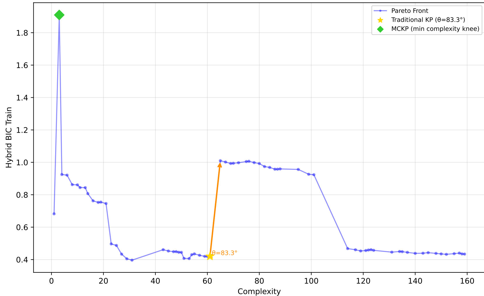
561_cpu - Run 9 - SVP - Hybrid BIC Train \lambda_1=0.90, \lambda_2=0.00, \lambda_3=0.30 | Difficulty: 0.55 | Method: mckp
