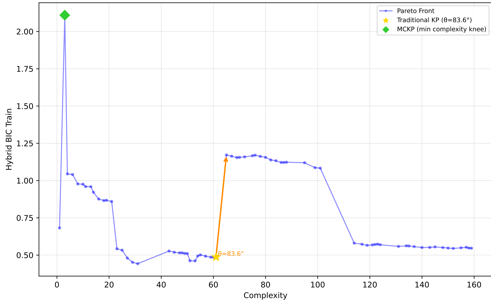
561_cpu - Run 9 - SVP - Hybrid BIC Train \lambda_1=1.00, \lambda_2=0.00, \lambda_3=0.40 | Difficulty: 0.55 | Method: mckp
