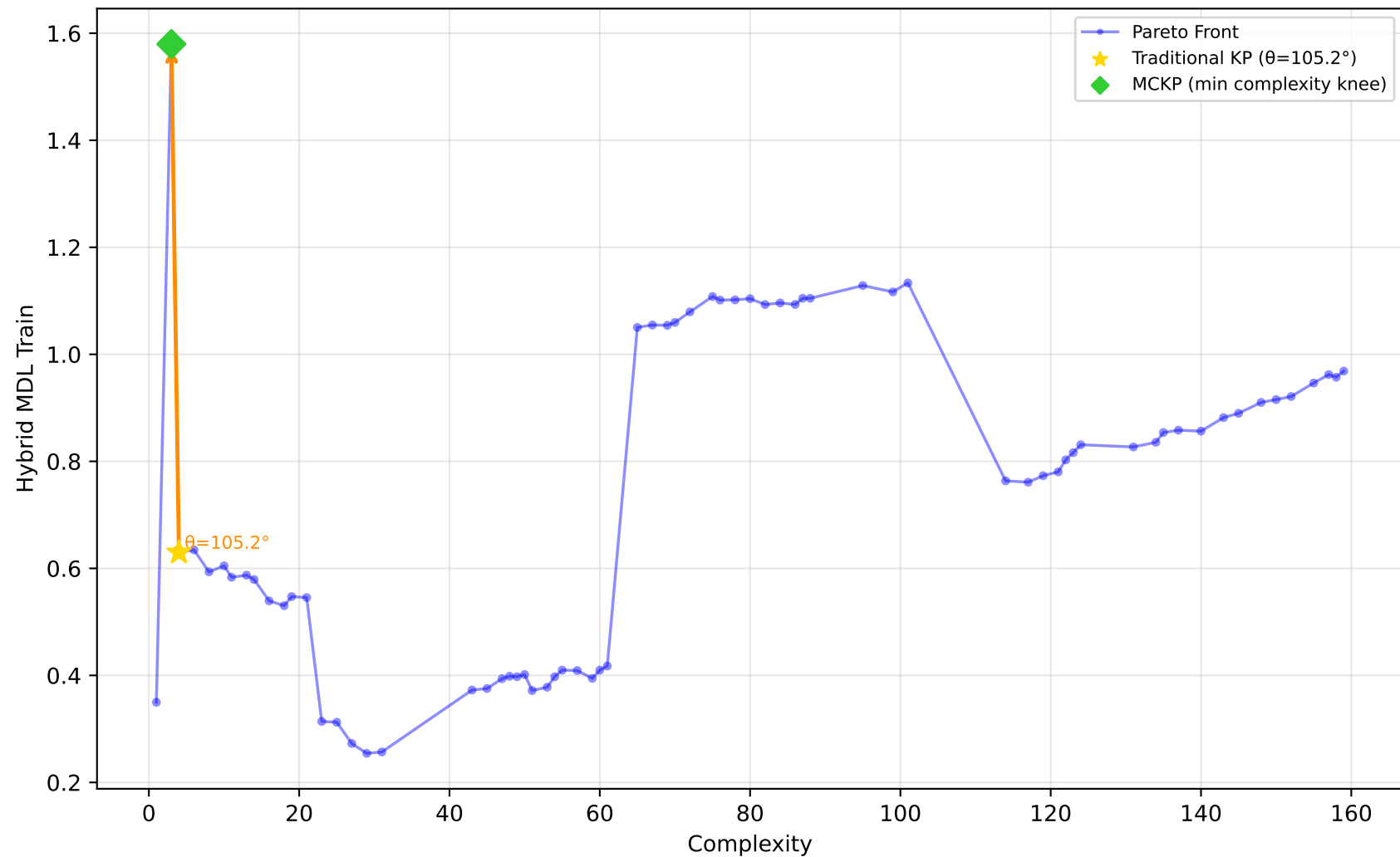
561_cpu - Run 9 - SVP - Hybrid MDL Train \lambda_1=0.90, \lambda_2=0.00, \lambda_3=0.30 | Difficulty: 0.55 | Method: mckp
