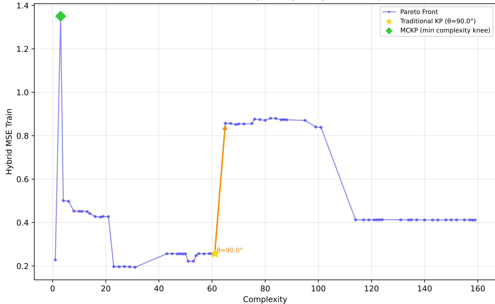
561_cpu - Run 9 - SVP - Hybrid MSE Train \lambda_1=0.90, \lambda_2=0.00, \lambda_3=0.30 | Difficulty: 0.55 | Method: mckp
