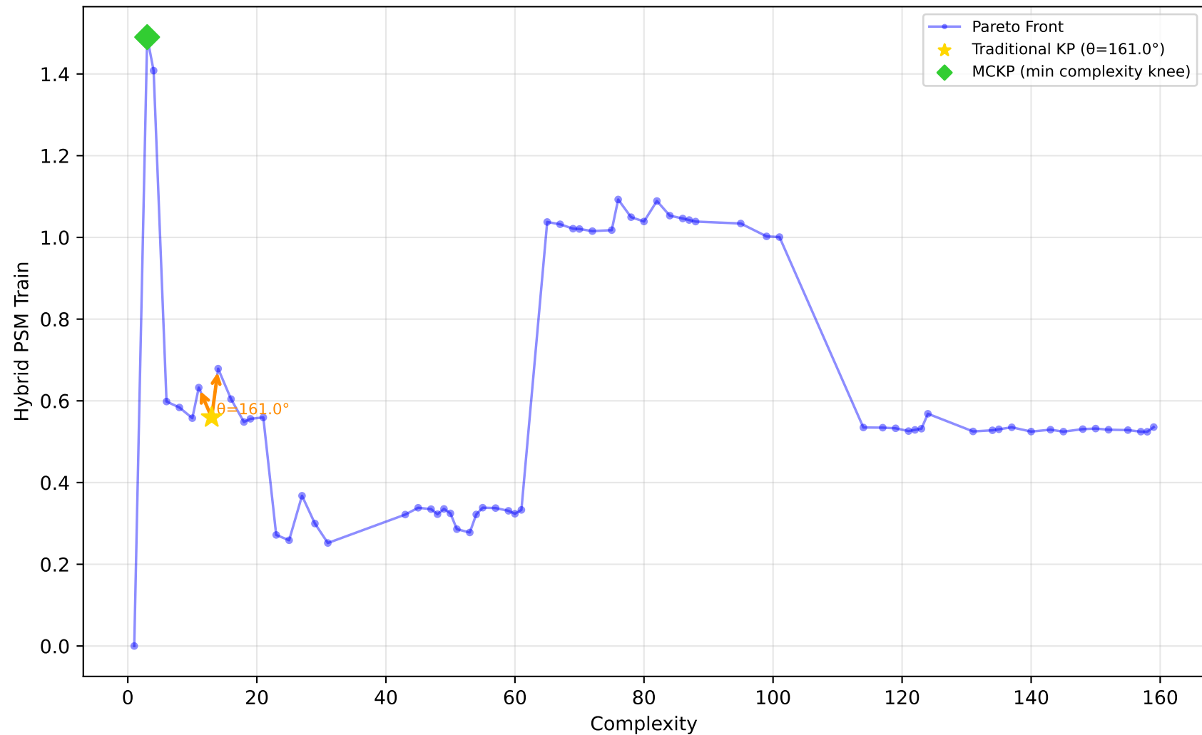
561_cpu - Run 9 - SVP - Hybrid PSM Train \lambda_1=1.00, \lambda_2=0.00, \lambda_3=0.40 | Difficulty: 0.55 | Method: mckp
