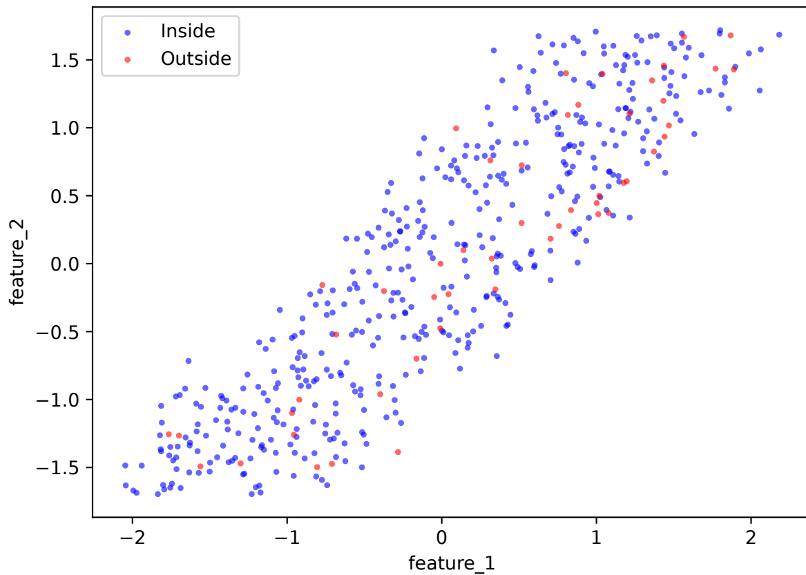
Plot with Bandwidth: 0.89
