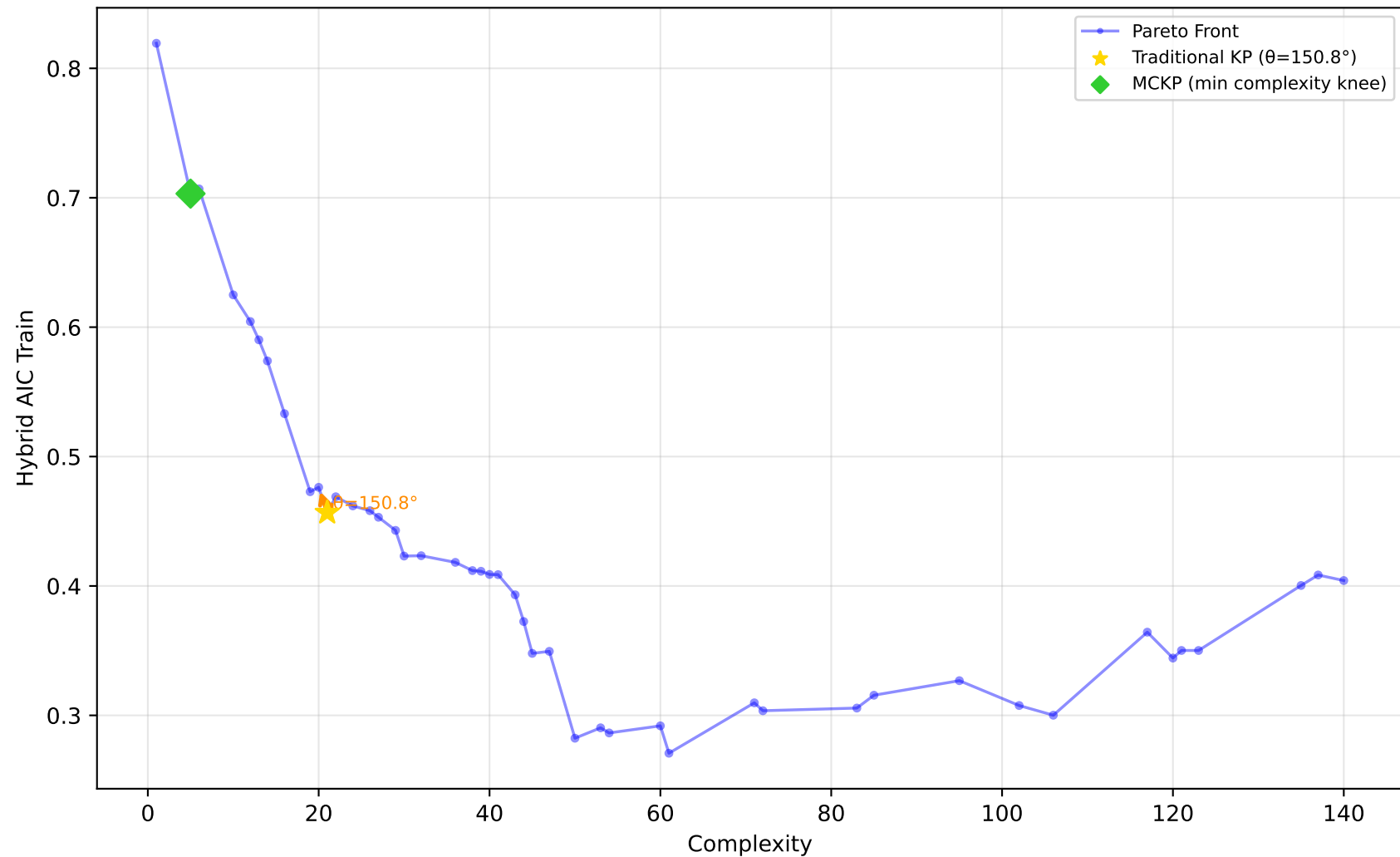
522_pm10 - Run 10 - MVP - Hybrid AIC Train \lambda_1=1.00, \lambda_2=0.00, \lambda_3=0.00 | Difficulty: 0.92 | Method: hmr
