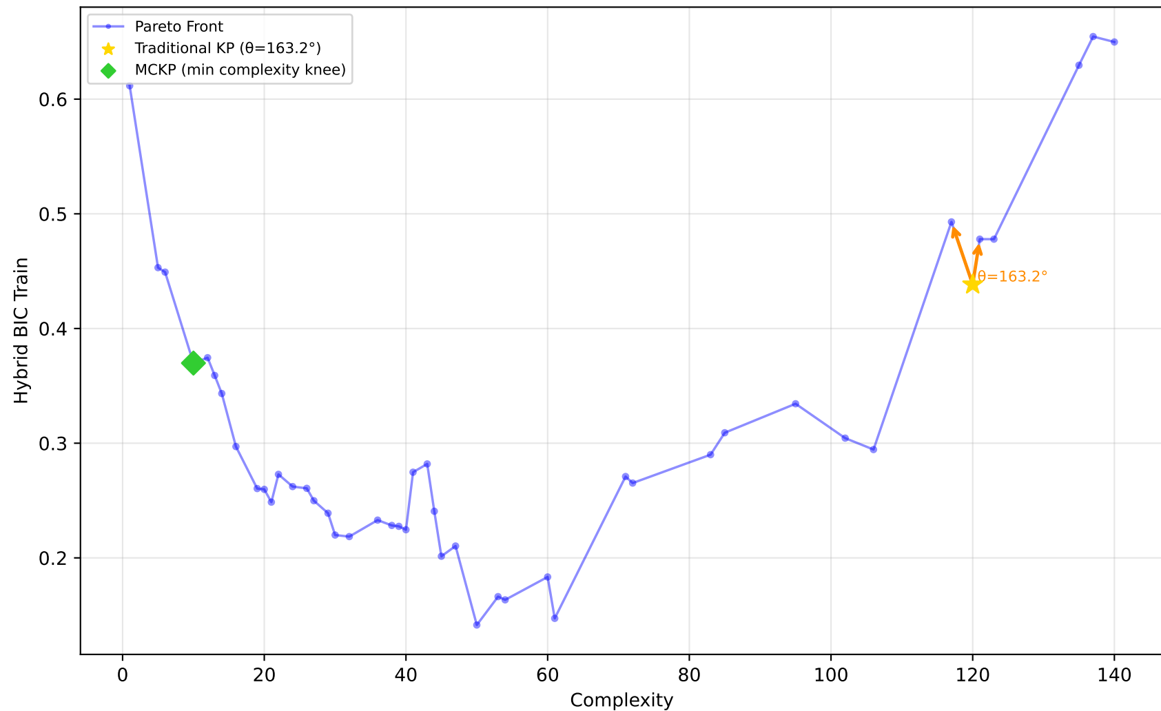
522_pm10 - Run 10 - MVP - Hybrid BIC Train \lambda_1=0.00, \lambda_2=0.90, \lambda_3=0.00 | Difficulty: 0.92 | Method: hmr
