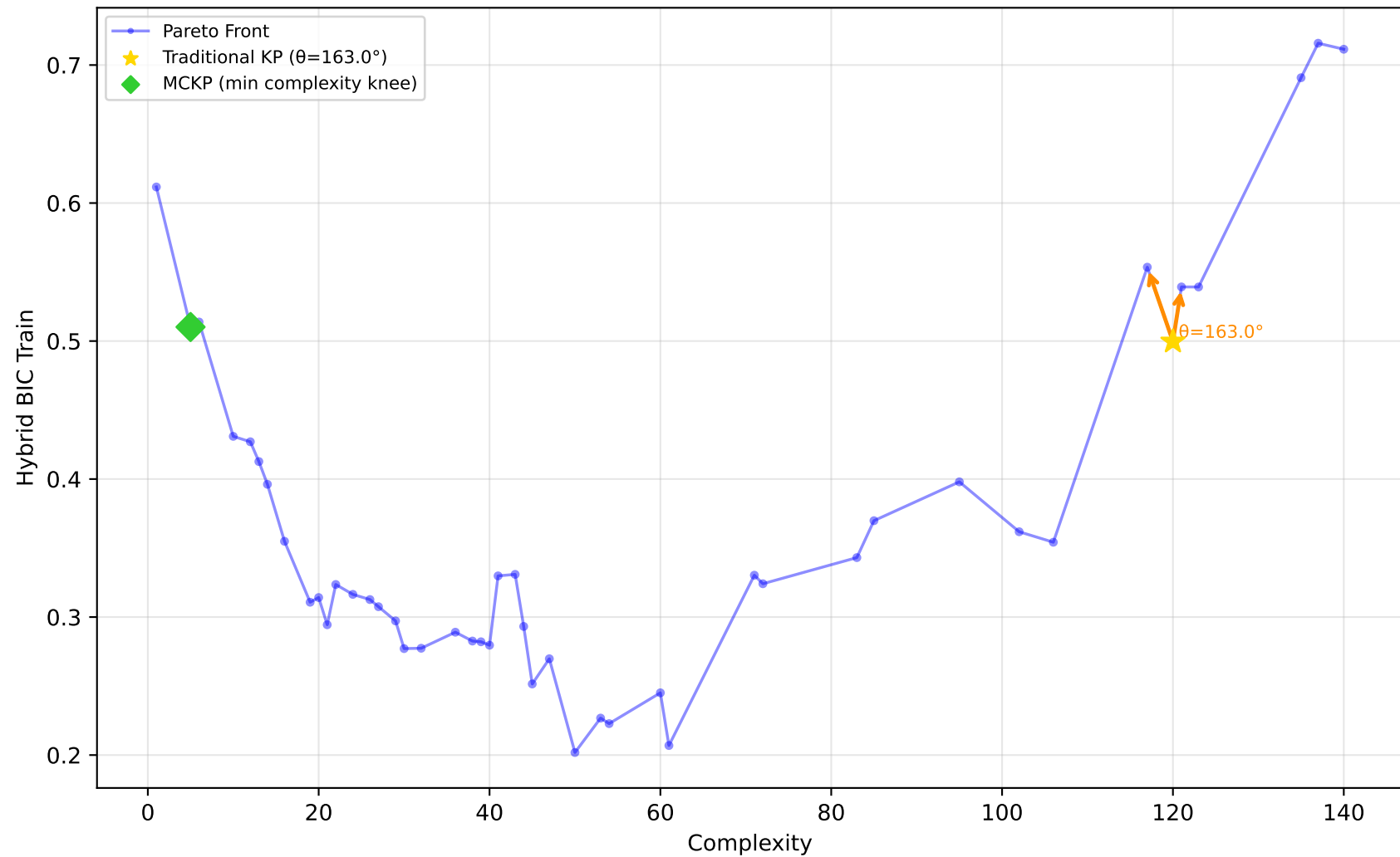
522_pm10 - Run 10 - MVP - Hybrid BIC Train \lambda_1=1.00, \lambda_2=0.00, \lambda_3=0.00 | Difficulty: 0.92 | Method: hmr
