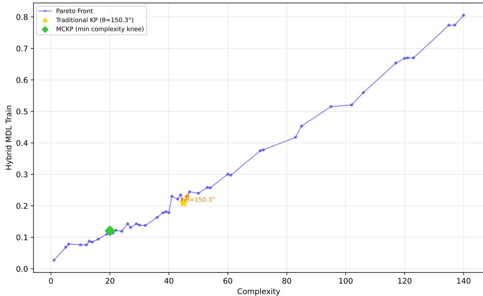
522_pm10 - Run 10 - MVP - Hybrid MDL Train \lambda_1=1.00, \lambda_2=0.00, \lambda_3=0.00 | Difficulty: 0.92 | Method: hmr
