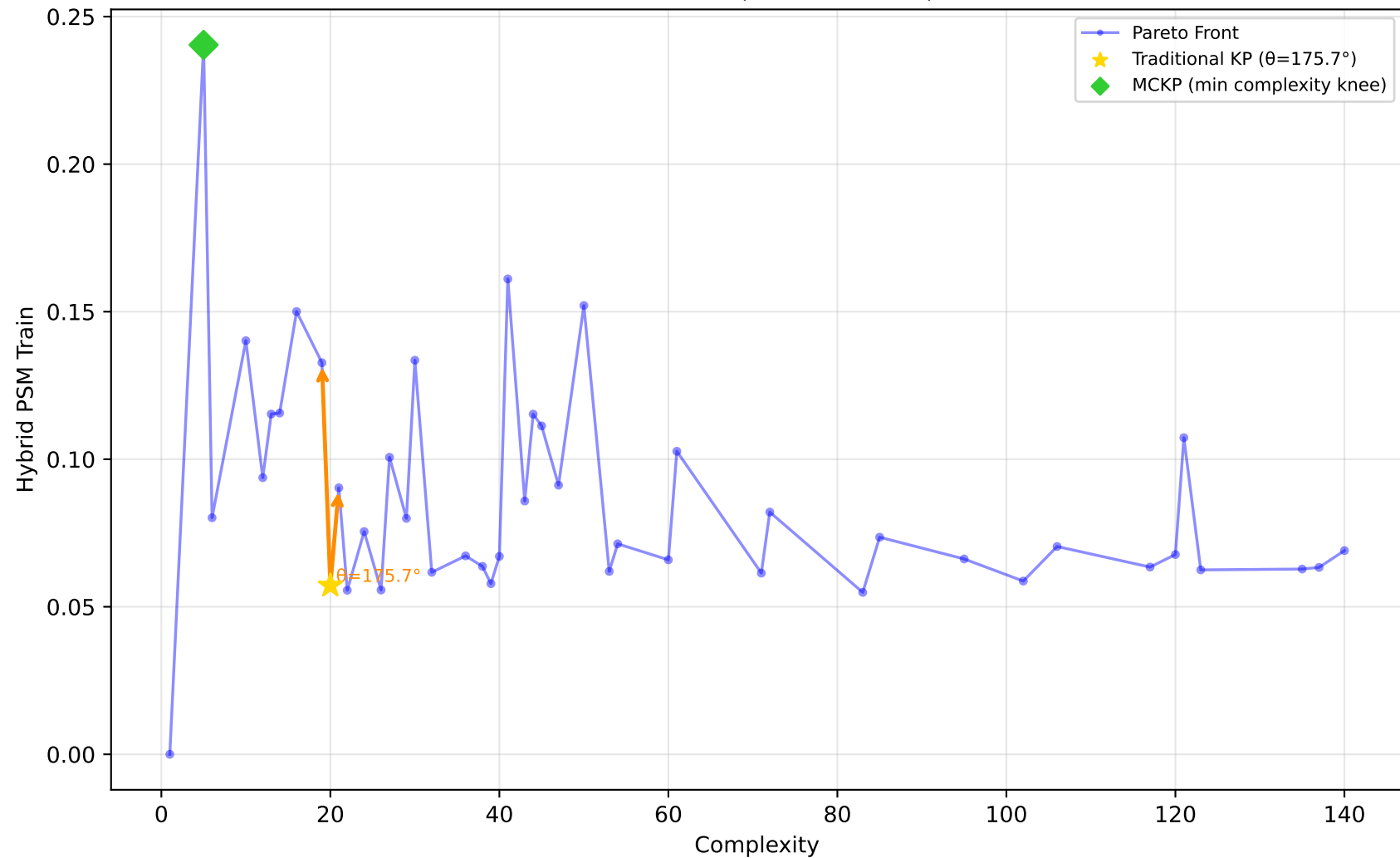
522_pm10 - Run 10 - MVP - Hybrid PSM Train \lambda_1=1.00, \lambda_2=0.00, \lambda_3=0.00 | Difficulty: 0.92 | Method: hmr
