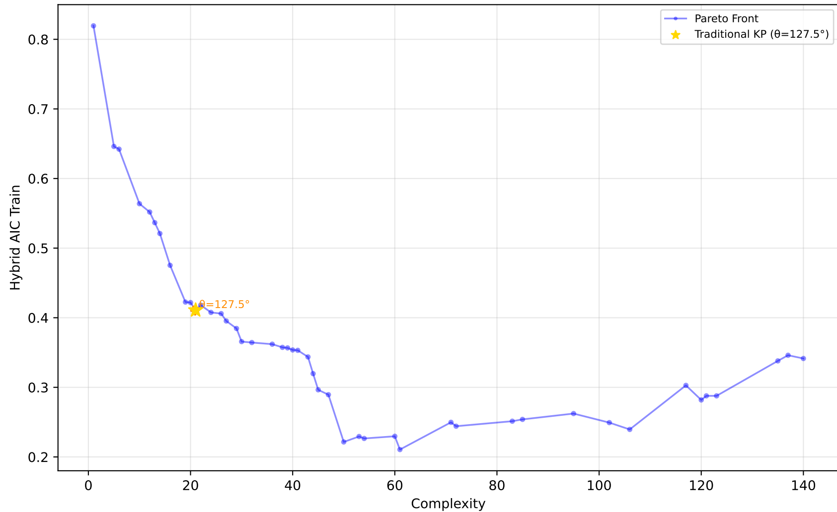
522_pm10 - Run 10 - SVP - Hybrid AIC Train \lambda_1=0.00, \lambda_2=0.10, \lambda_3=0.00 | Difficulty: 0.92 | Method: hmr
