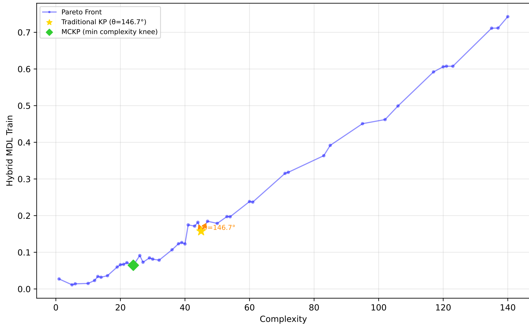
522_pm10 - Run 10 - SVP - Hybrid MDL Train \lambda_1=0.00, \lambda_2=0.10, \lambda_3=0.00 | Difficulty: 0.92 | Method: hmr
