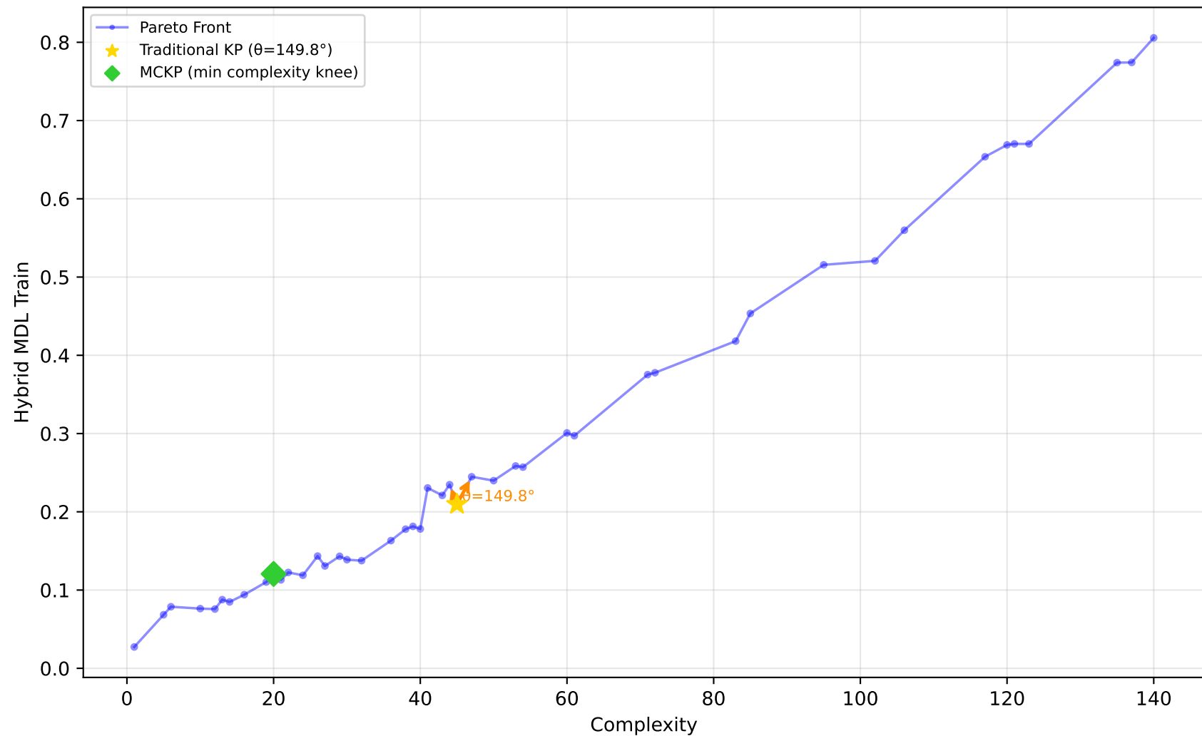
522_pm10 - Run 10 - SVP - Hybrid MDL Train \lambda_1=1.00, \lambda_2=0.00, \lambda_3=0.90 | Difficulty: 0.92 | Method: hmr
