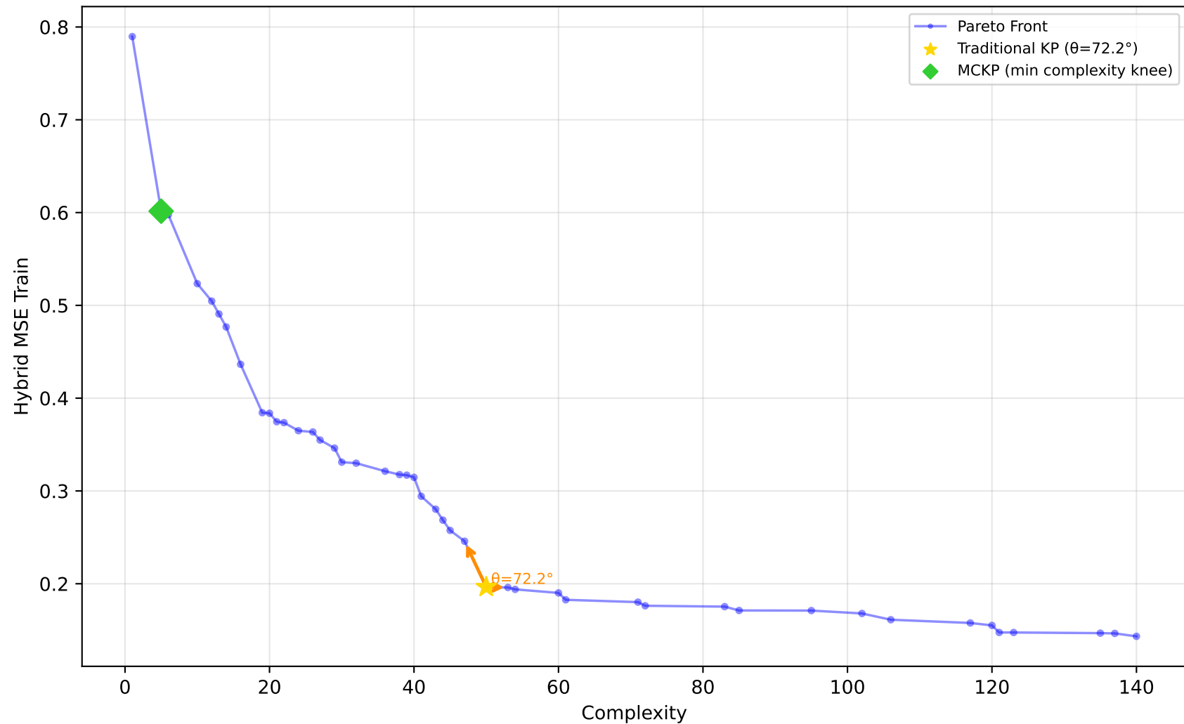
522_pm10 - Run 10 - SVP - Hybrid MSE Train \lambda_1=0.00, \lambda_2=0.10, \lambda_3=0.00 | Difficulty: 0.92 | Method: hmr
