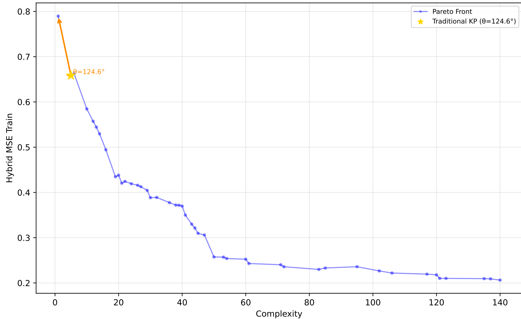
522_pm10 - Run 10 - SVP - Hybrid MSE Train \lambda_1=1.00, \lambda_2=0.00, \lambda_3=0.90 | Difficulty: 0.92 | Method: hmr
