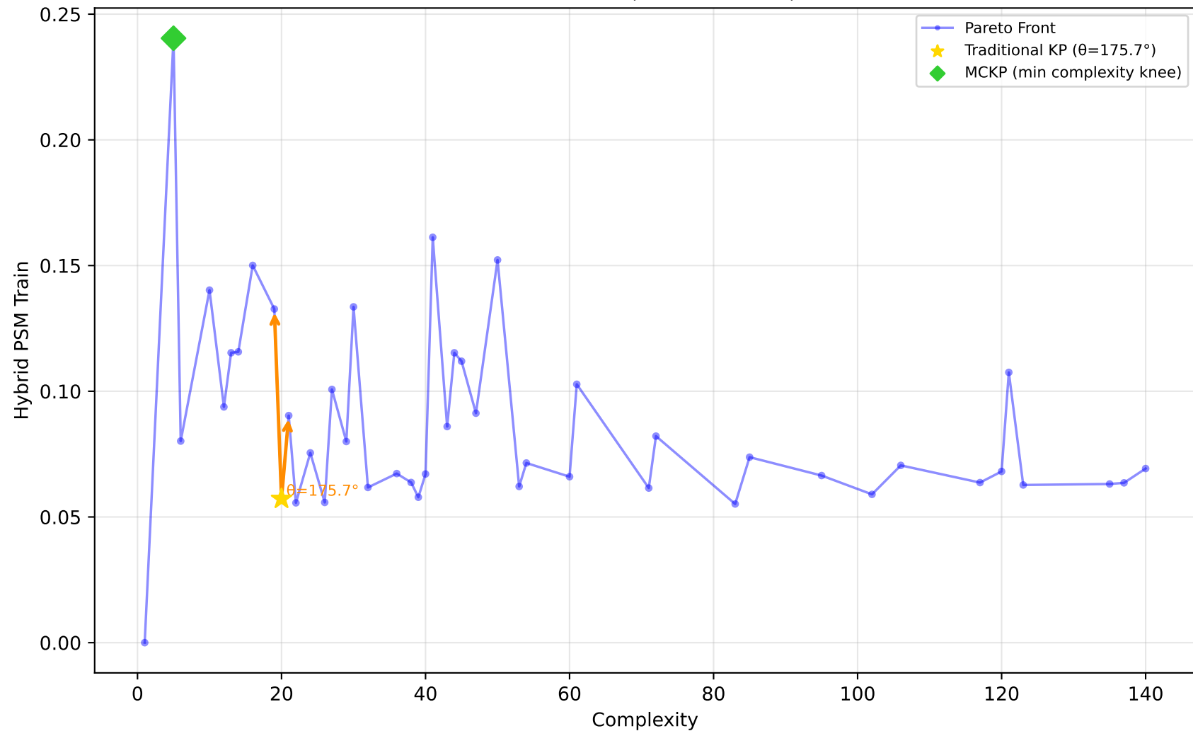
522_pm10 - Run 10 - SVP - Hybrid PSM Train \lambda_1=1.00, \lambda_2=0.00, \lambda_3=0.90 | Difficulty: 0.92 | Method: hmr
