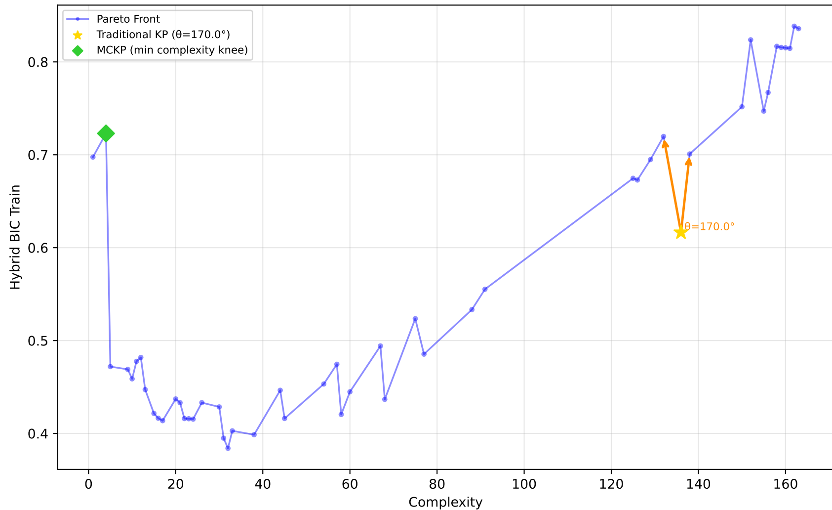
522_pm10 - Run 11 - MVP - Hybrid BIC Train \lambda_1=0.00, \lambda_2=0.90, \lambda_3=0.00 | Difficulty: 1.00 | Method: hmr
