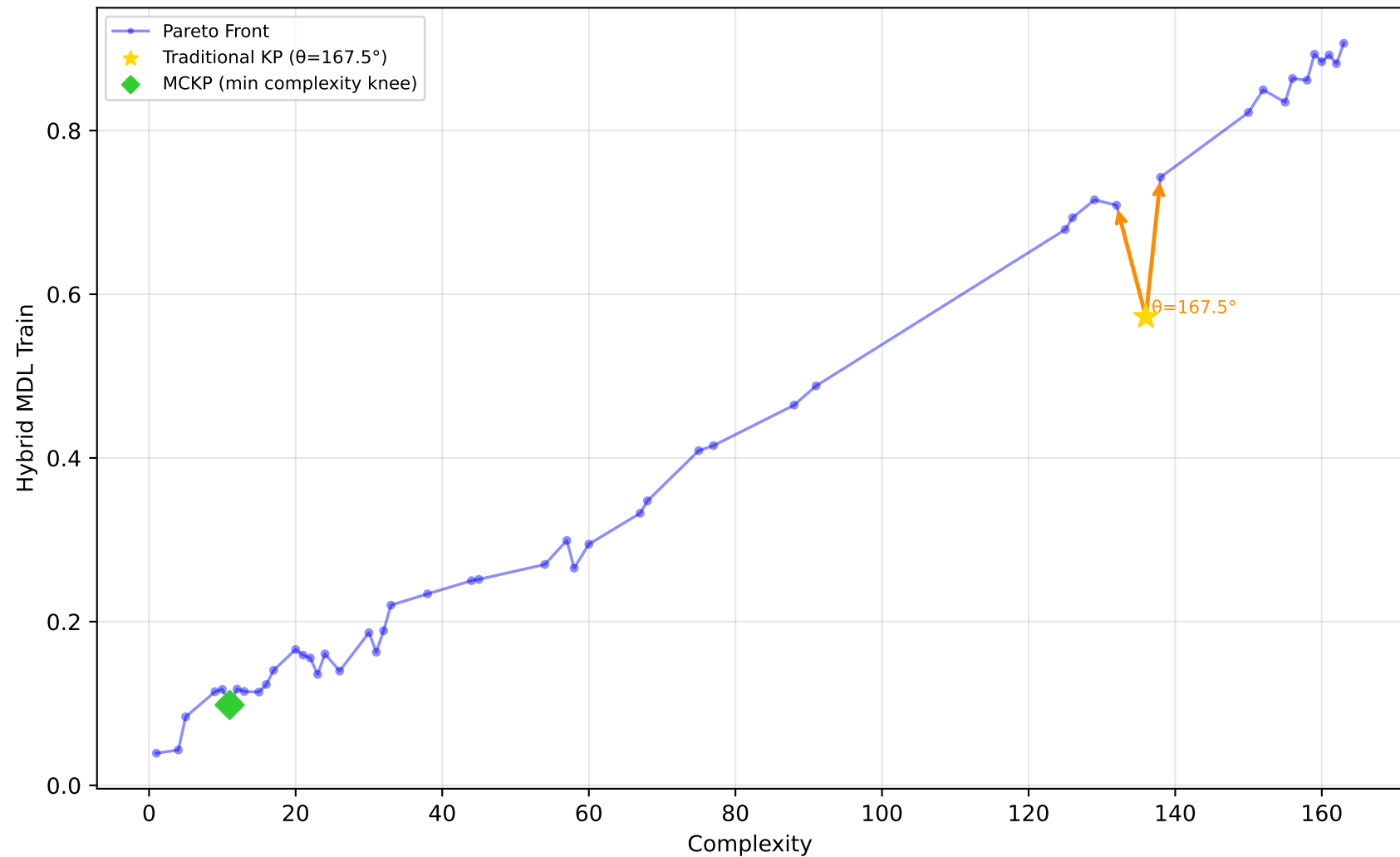
522_pm10 - Run 11 - MVP - Hybrid MDL Train \lambda_1=1.00, \lambda_2=0.00, \lambda_3=0.00 | Difficulty: 1.00 | Method: hmr
