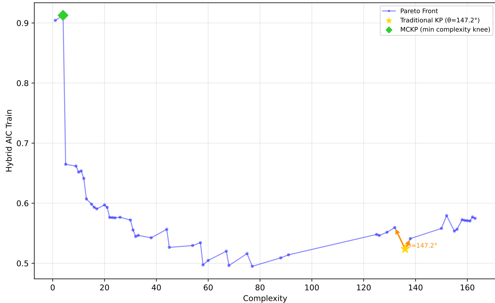
522_pm10 - Run 11 - SVP - Hybrid AIC Train \lambda_1=0.00, \lambda_2=0.10, \lambda_3=0.00 | Difficulty: 1.00 | Method: hmr
