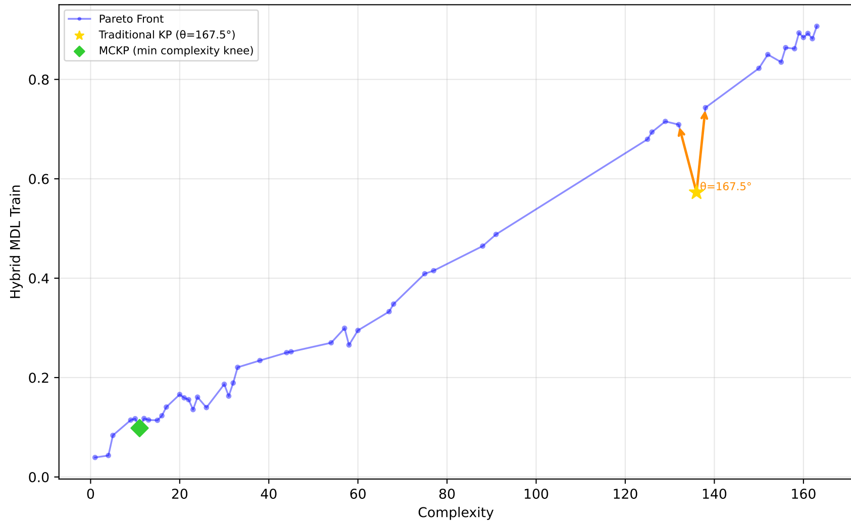
522_pm10 - Run 11 - SVP - Hybrid MDL Train \lambda_1=1.00, \lambda_2=0.00, \lambda_3=0.90 | Difficulty: 1.00 | Method: hmr
