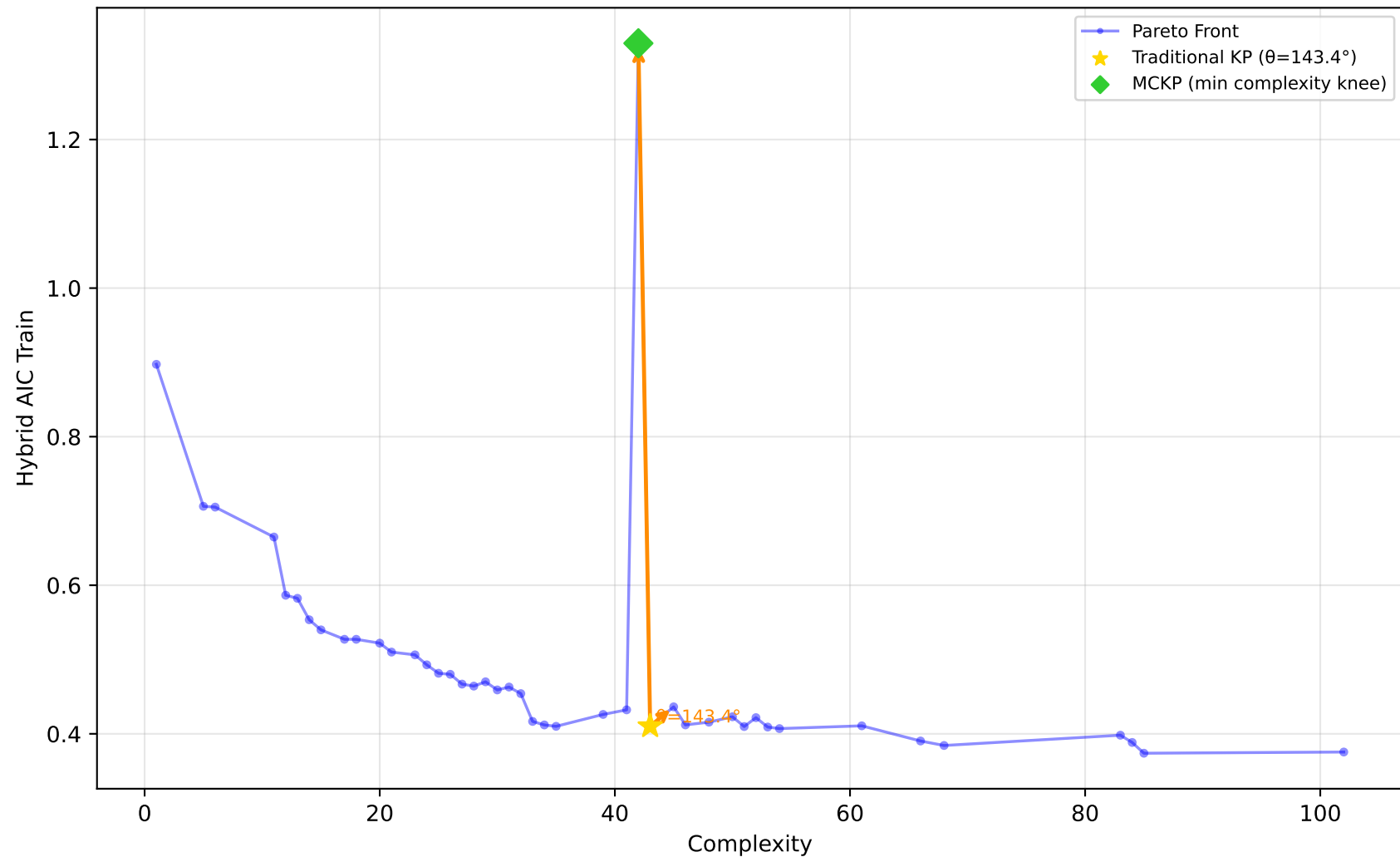
522_pm10 - Run 12 - MVP - Hybrid AIC Train \lambda_1=0.00, \lambda_2=0.90, \lambda_3=0.00 | Difficulty: 1.00 | Method: hmr
