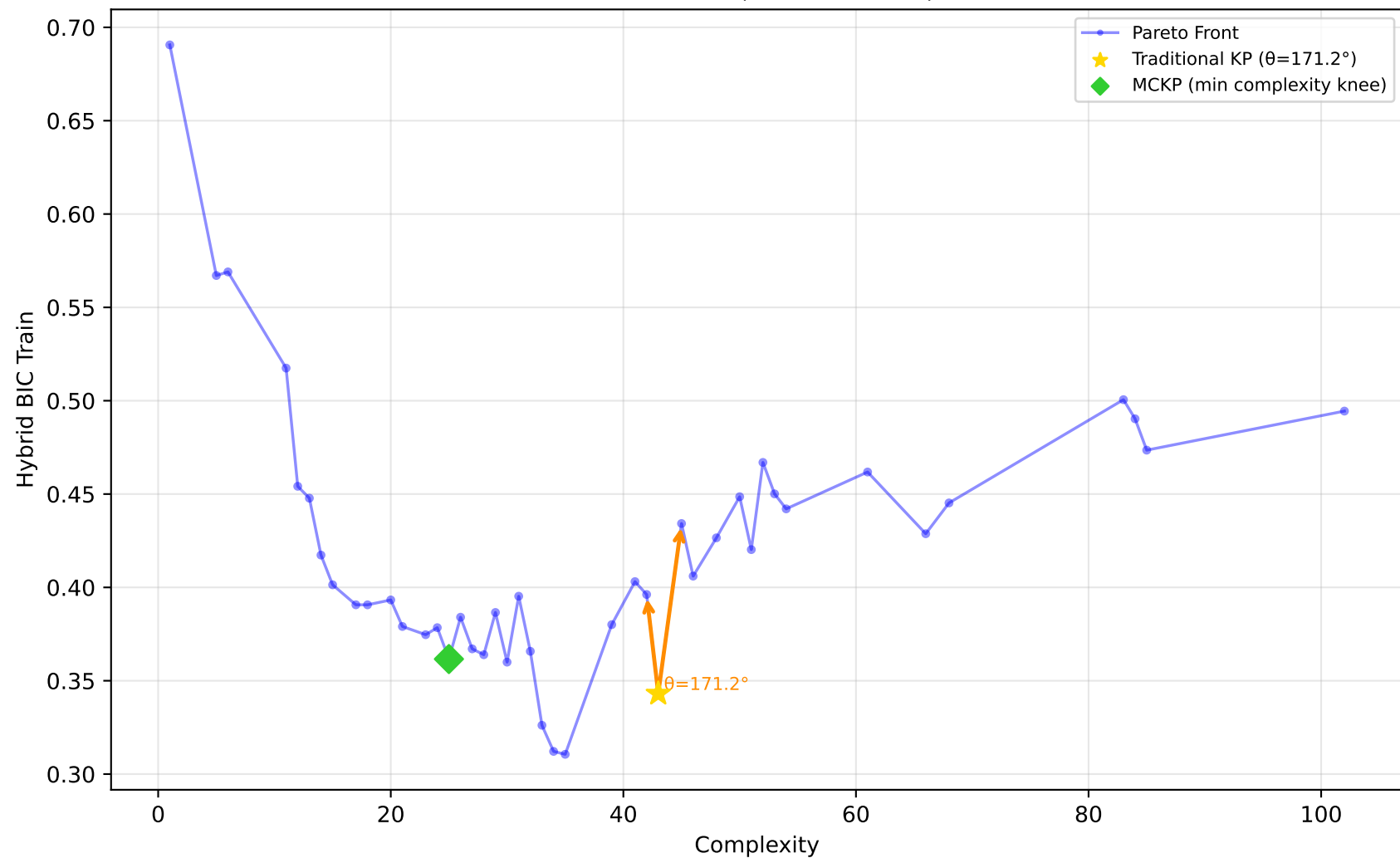
522_pm10 - Run 12 - MVP - Hybrid BIC Train \lambda_1=1.00, \lambda_2=0.00, \lambda_3=0.00 | Difficulty: 1.00 | Method: hmr
