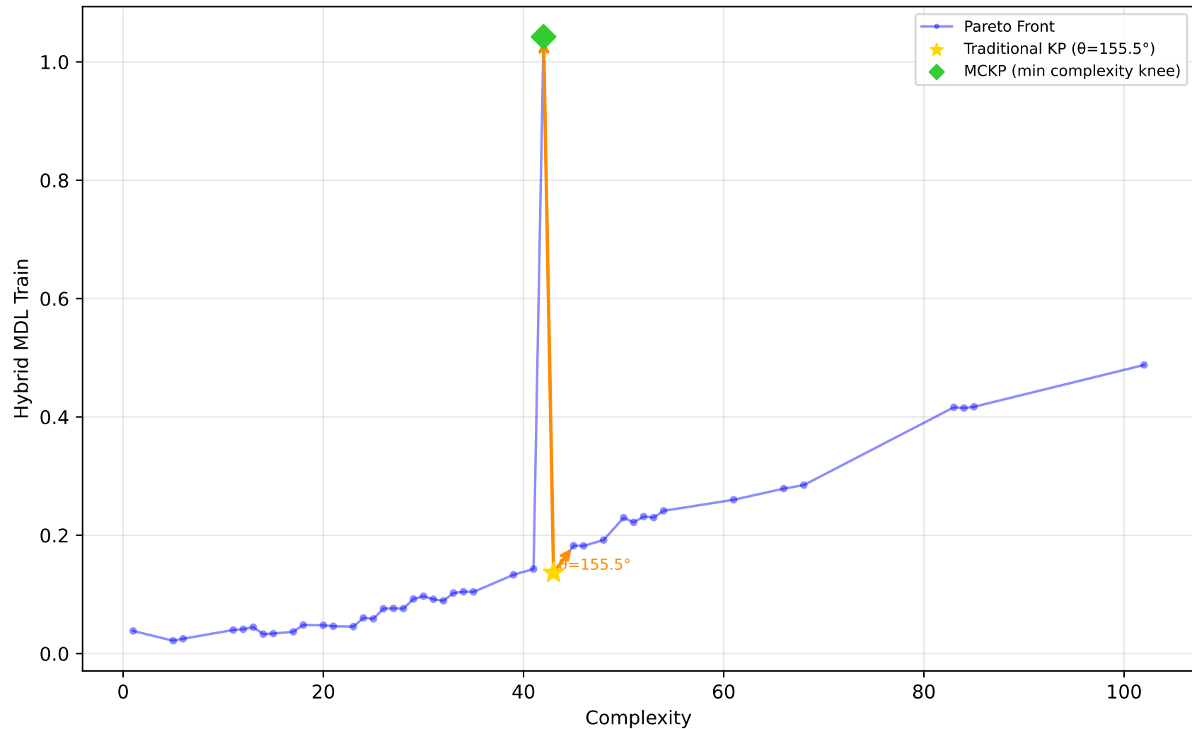
522_pm10 - Run 12 - MVP - Hybrid MDL Train \lambda_1=0.00, \lambda_2=0.90, \lambda_3=0.00 | Difficulty: 1.00 | Method: hmr
