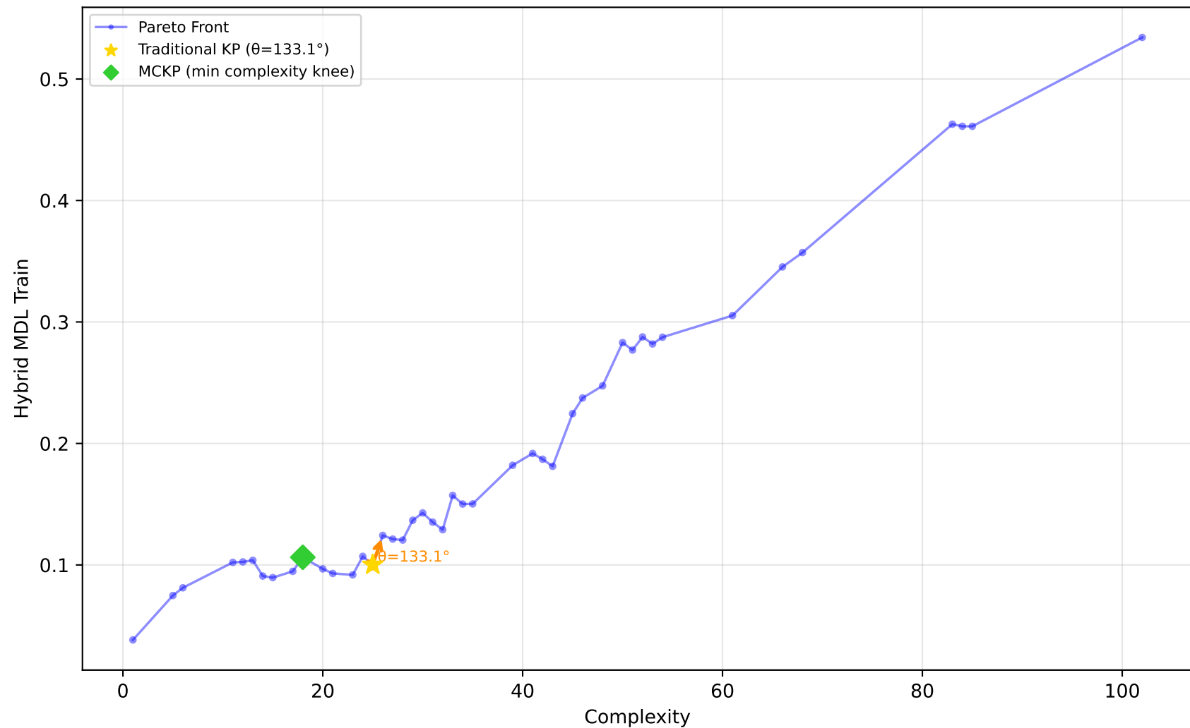
522_pm10 - Run 12 - MVP - Hybrid MDL Train \lambda_1=1.00, \lambda_2=0.00, \lambda_3=0.00 | Difficulty: 1.00 | Method: hmr
