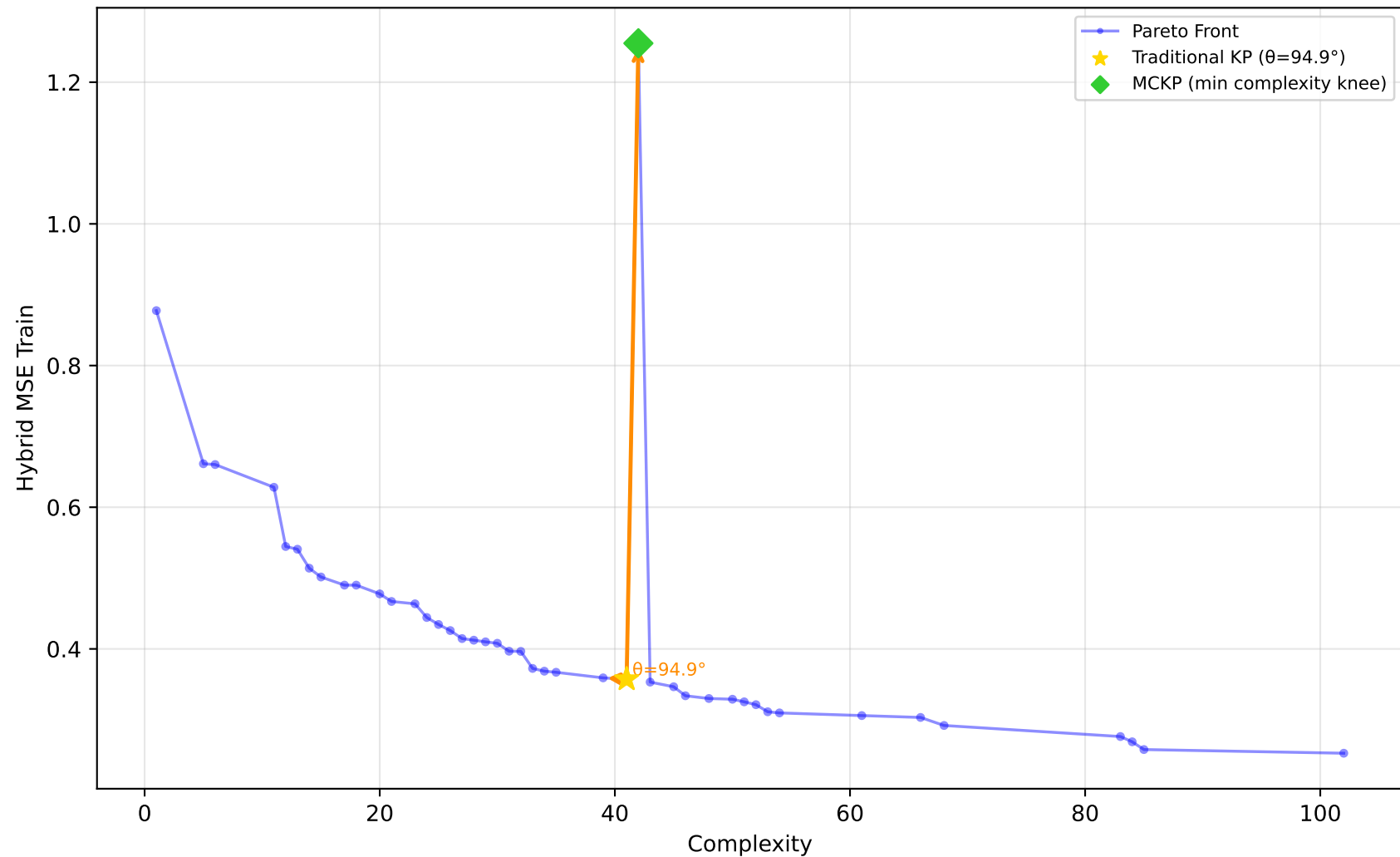
522_pm10 - Run 12 - MVP - Hybrid MSE Train \lambda_1=0.00, \lambda_2=0.90, \lambda_3=0.00 | Difficulty: 1.00 | Method: hmr
