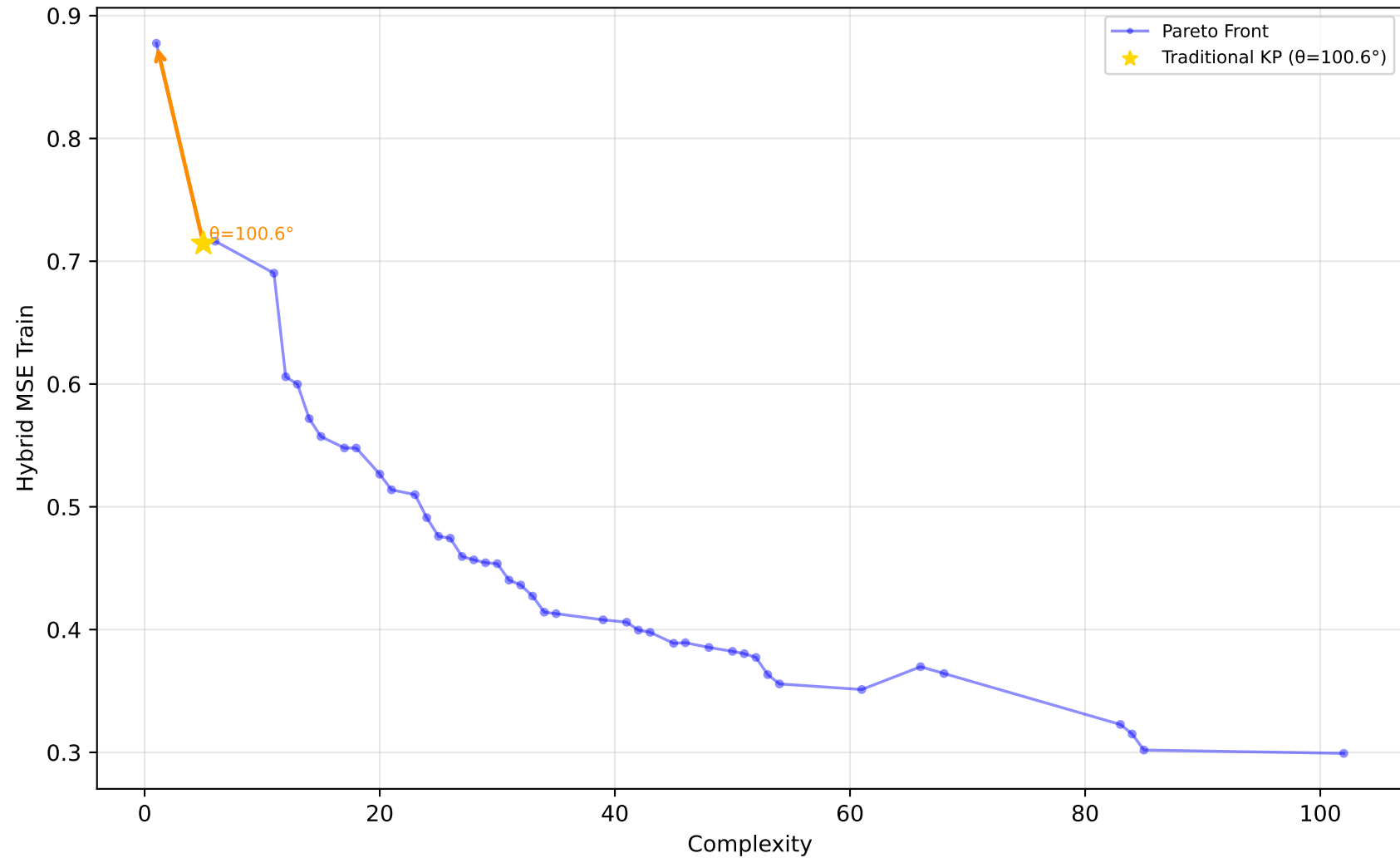
522_pm10 - Run 12 - MVP - Hybrid MSE Train \lambda_1=1.00, \lambda_2=0.00, \lambda_3=0.00 | Difficulty: 1.00 | Method: hmr
