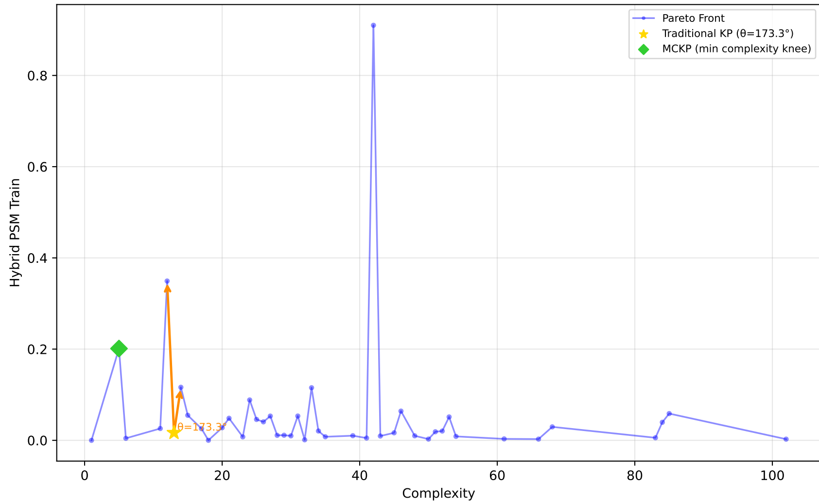
522_pm10 - Run 12 - MVP - Hybrid PSM Train \lambda_1=0.00, \lambda_2=0.90, \lambda_3=0.00 | Difficulty: 1.00 | Method: hmr
