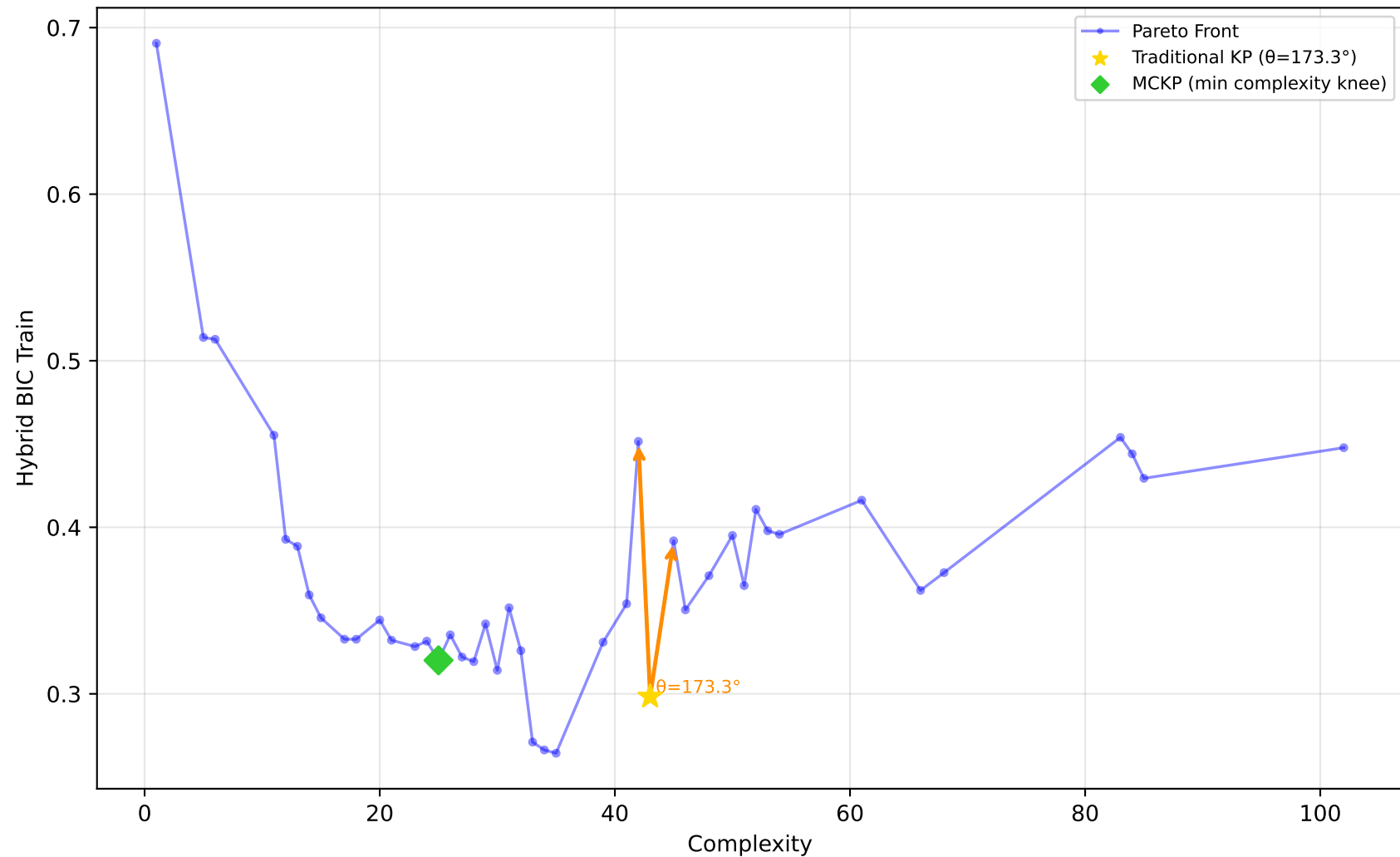
522_pm10 - Run 12 - SVP - Hybrid BIC Train \lambda_1=0.00, \lambda_2=0.10, \lambda_3=0.00 | Difficulty: 1.00 | Method: hmr
