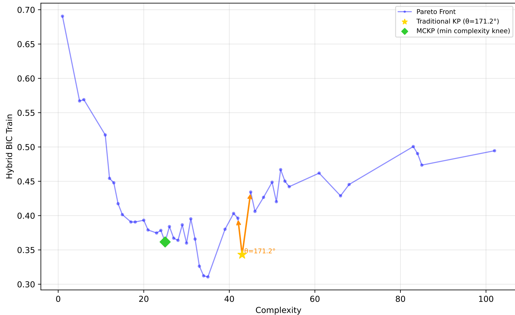
522_pm10 - Run 12 - SVP - Hybrid BIC Train \lambda_1=1.00, \lambda_2=0.00, \lambda_3=0.90 | Difficulty: 1.00 | Method: hmr
