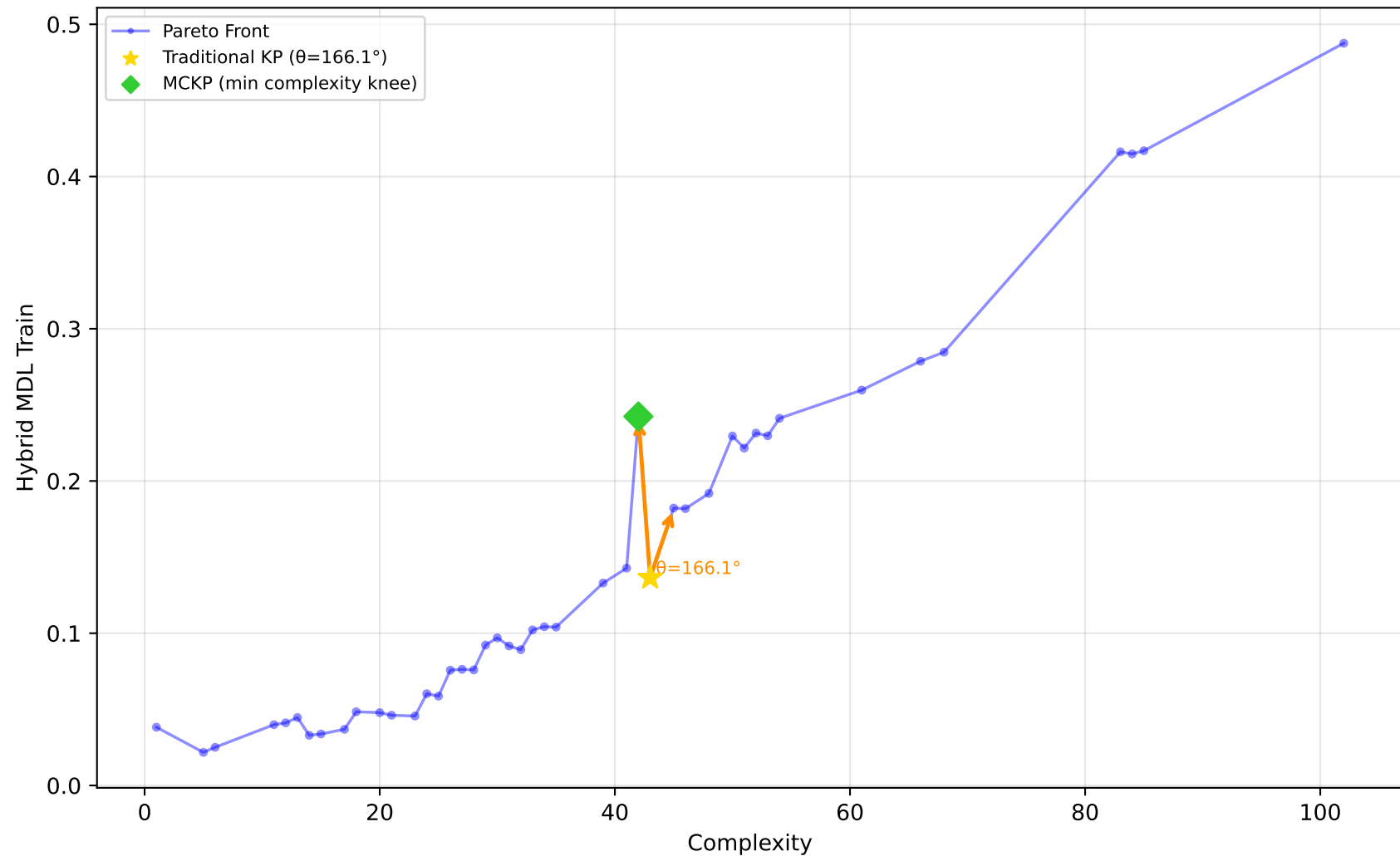
522_pm10 - Run 12 - SVP - Hybrid MDL Train \lambda_1=0.00, \lambda_2=0.10, \lambda_3=0.00 | Difficulty: 1.00 | Method: hmr
