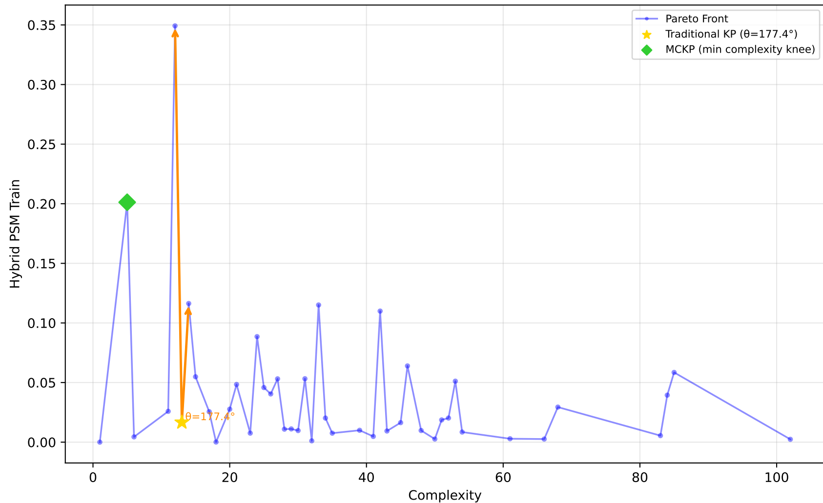
522_pm10 - Run 12 - SVP - Hybrid PSM Train \lambda_1=0.00, \lambda_2=0.10, \lambda_3=0.00 | Difficulty: 1.00 | Method: hmr
