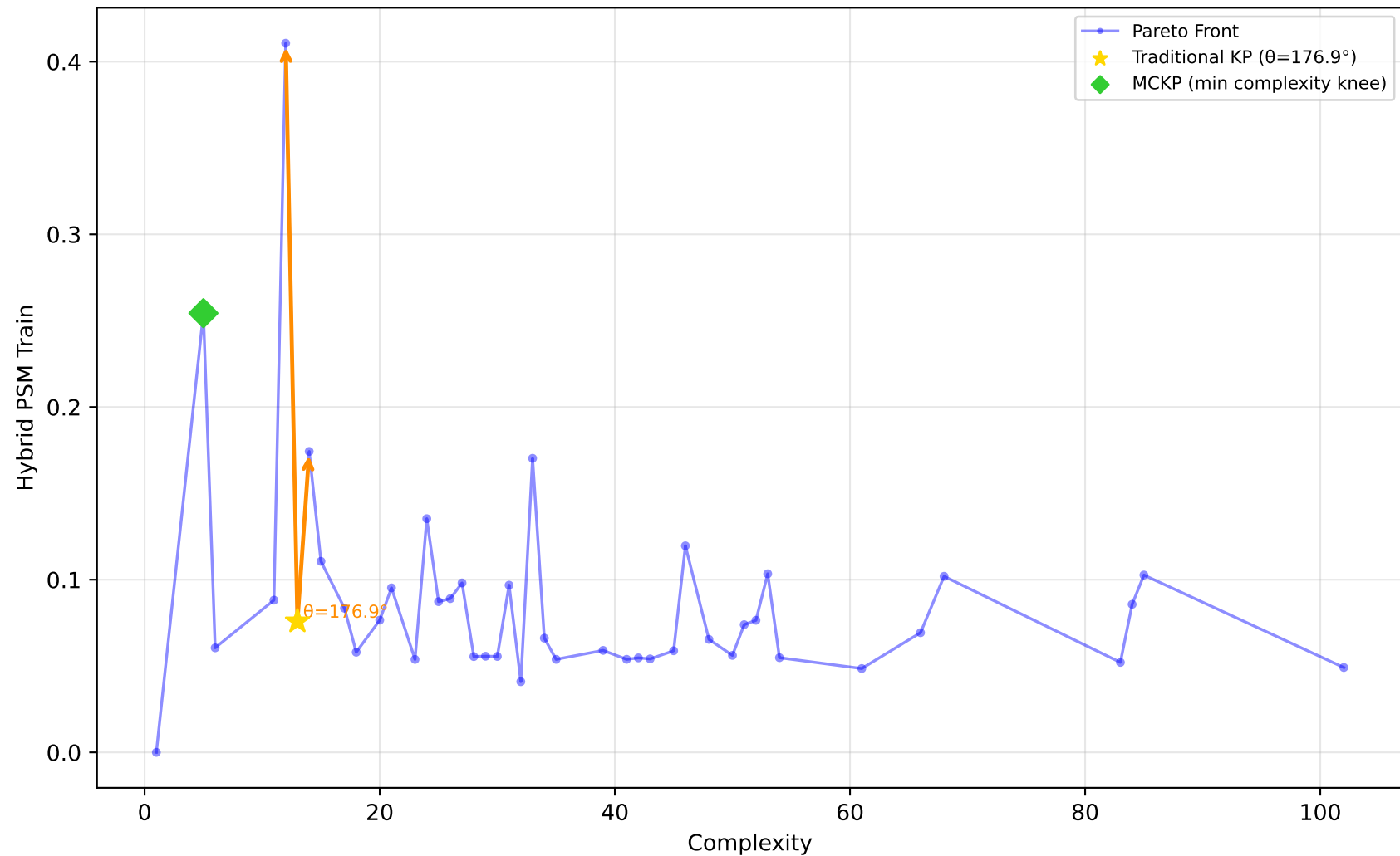
522_pm10 - Run 12 - SVP - Hybrid PSM Train \lambda_1=1.00, \lambda_2=0.00, \lambda_3=0.90 | Difficulty: 1.00 | Method: hmr
