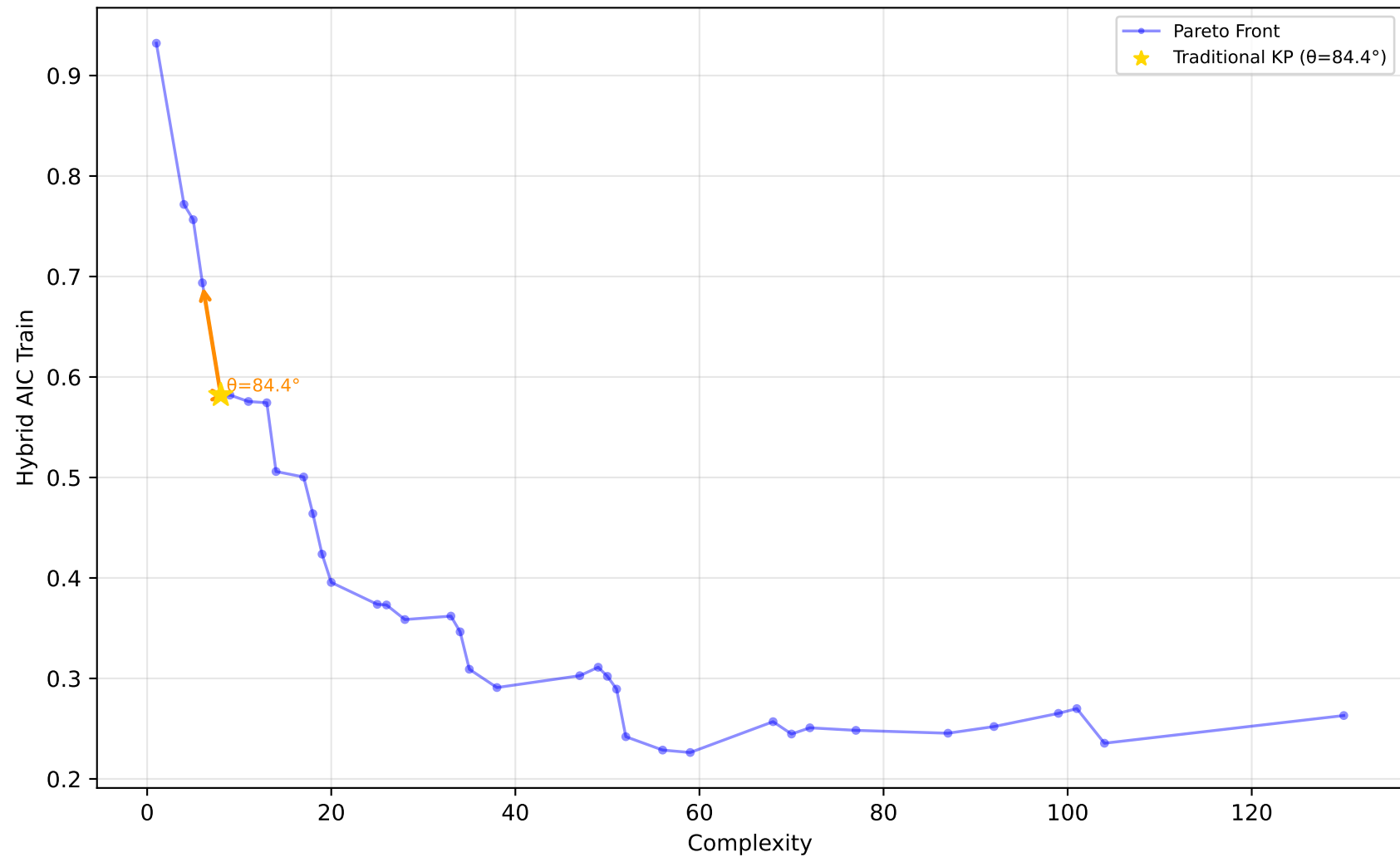
522_pm10 - Run 13 - MVP - Hybrid AIC Train \lambda_1=0.00, \lambda_2=0.90, \lambda_3=0.00 | Difficulty: 0.95 | Method: hmr
