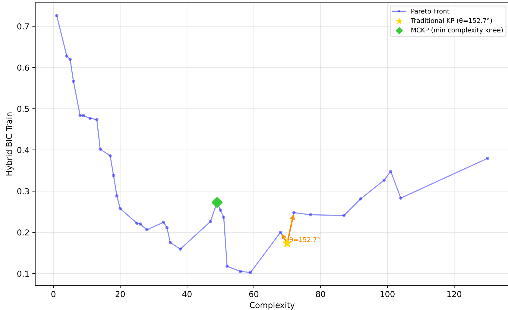
522_pm10 - Run 13 - MVP - Hybrid BIC Train \lambda_1=1.00, \lambda_2=0.00, \lambda_3=0.00 | Difficulty: 0.95 | Method: hmr
