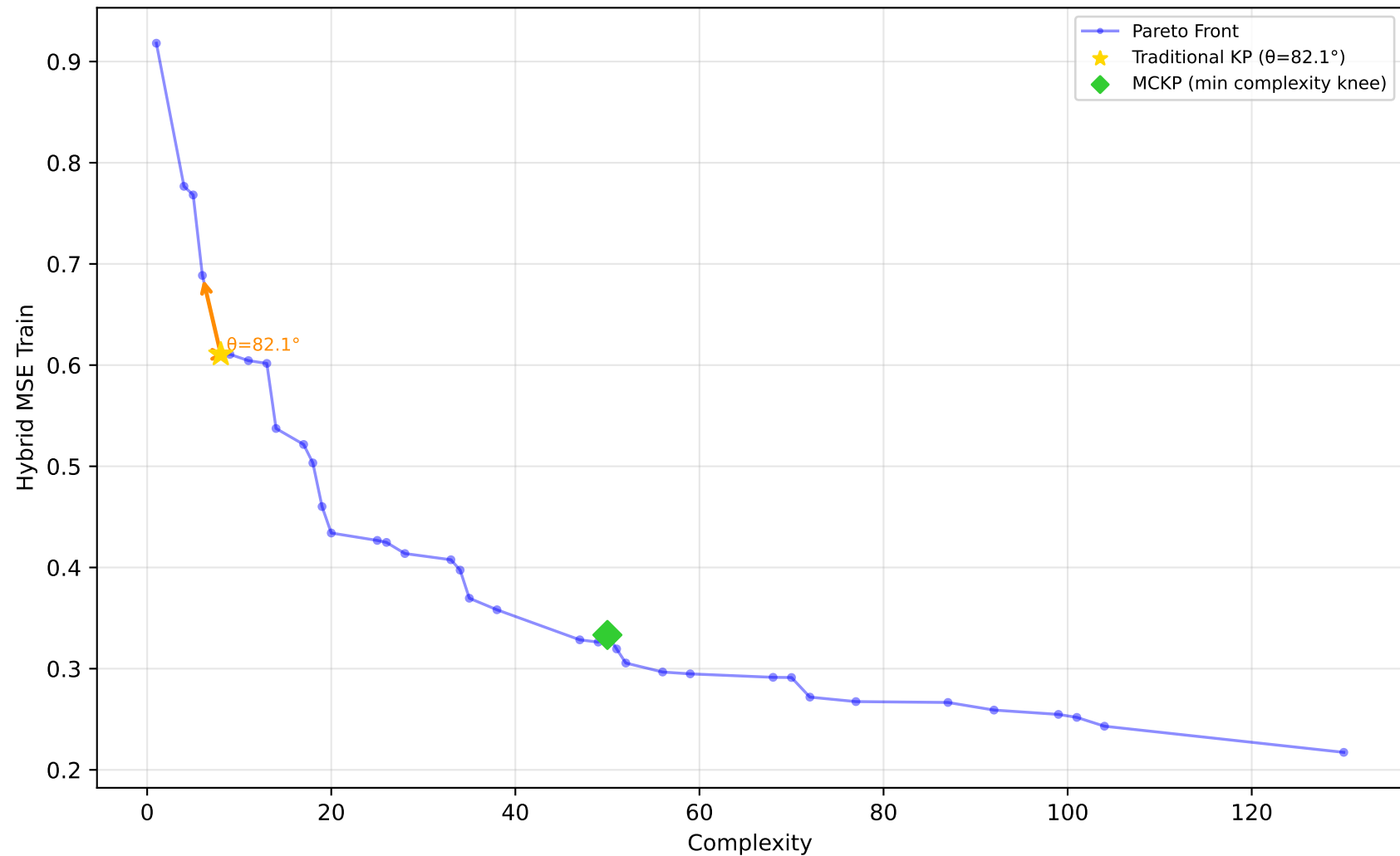
522_pm10 - Run 13 - MVP - Hybrid MSE Train \lambda_1=1.00, \lambda_2=0.00, \lambda_3=0.00 | Difficulty: 0.95 | Method: hmr
