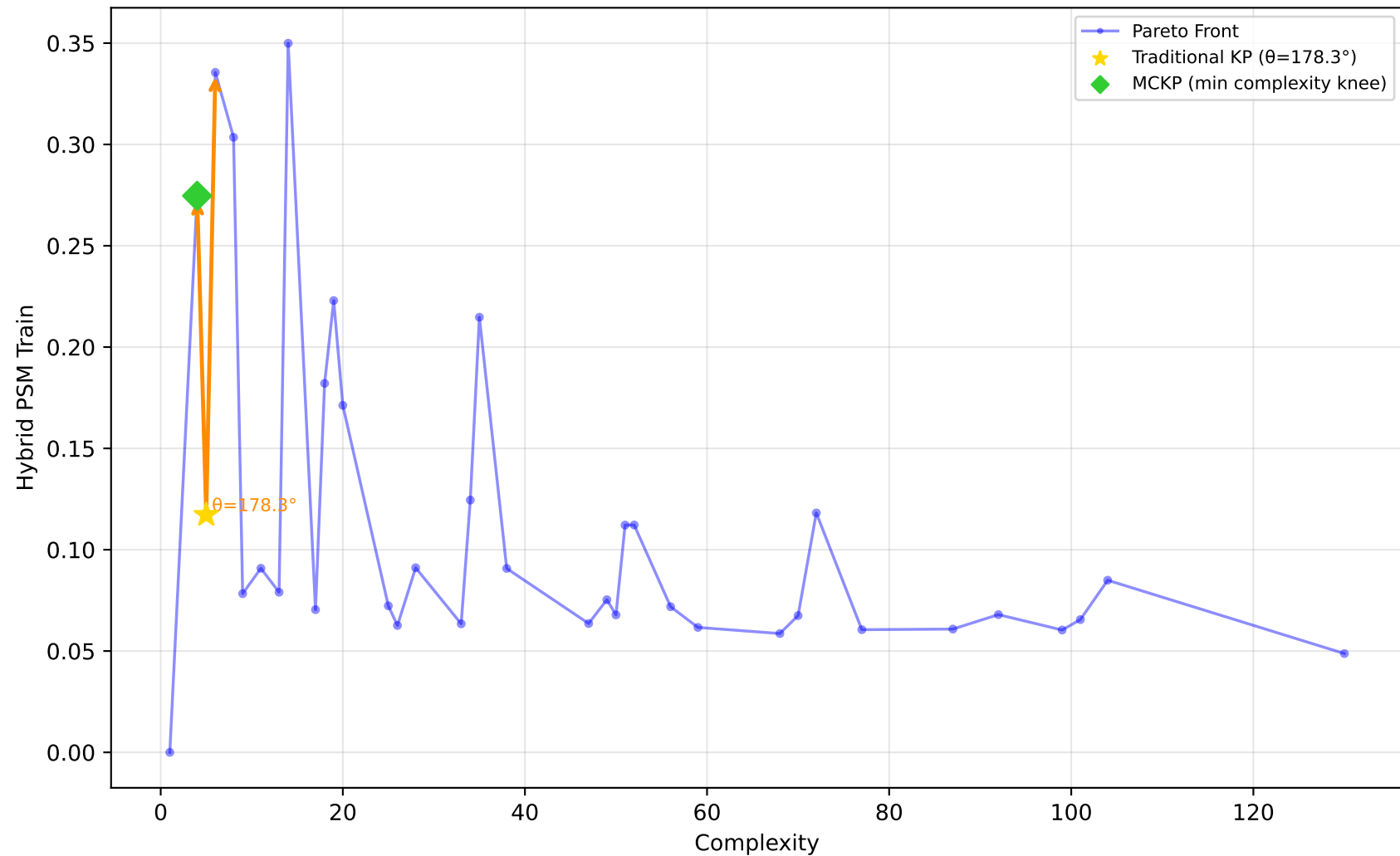
522_pm10 - Run 13 - MVP - Hybrid PSM Train \lambda_1=1.00, \lambda_2=0.00, \lambda_3=0.00 | Difficulty: 0.95 | Method: hmr
