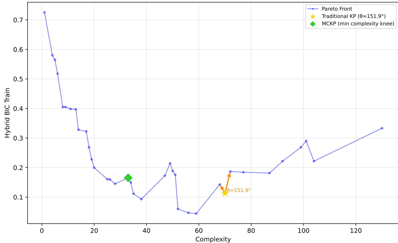
522_pm10 - Run 13 - SVP - Hybrid BIC Train \lambda_1=0.00, \lambda_2=0.10, \lambda_3=0.00 | Difficulty: 0.95 | Method: hmr
