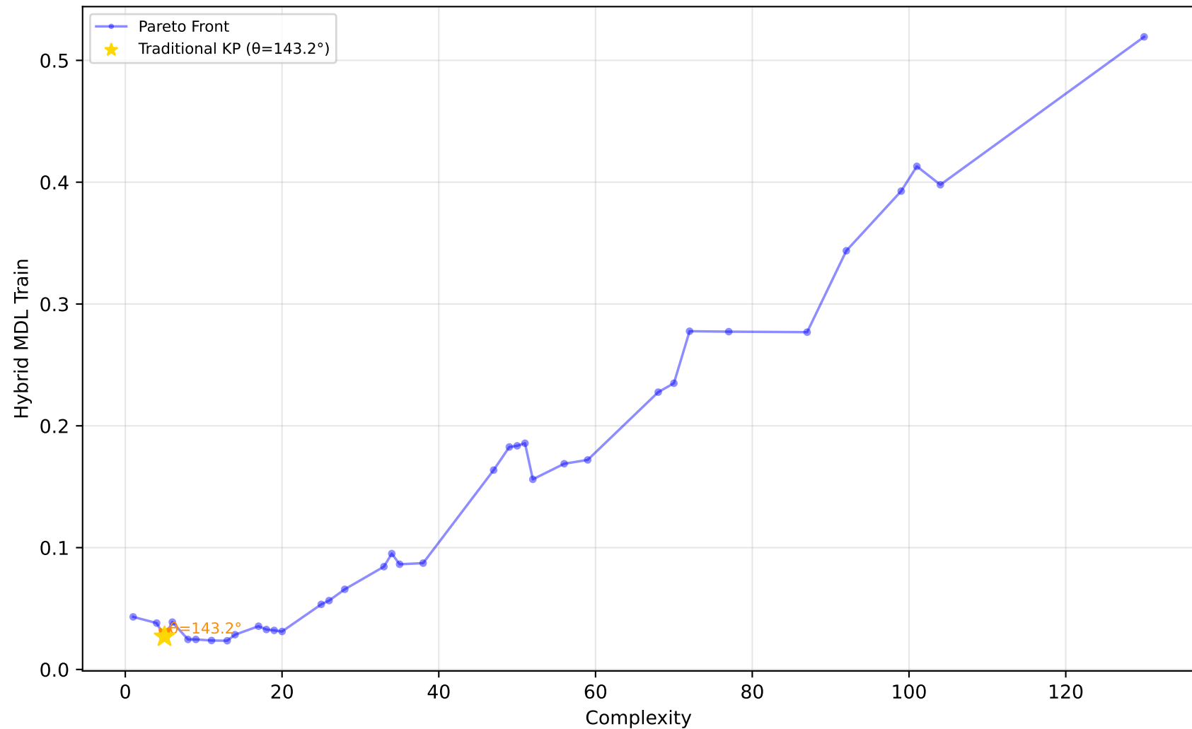
522_pm10 - Run 13 - SVP - Hybrid MDL Train \lambda_1=0.00, \lambda_2=0.10, \lambda_3=0.00 | Difficulty: 0.95 | Method: hmr
