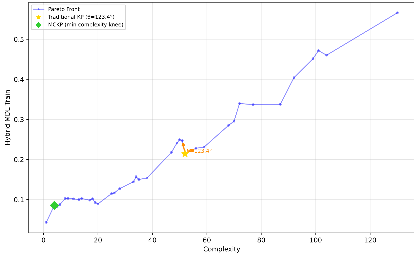
522_pm10 - Run 13 - SVP - Hybrid MDL Train \lambda_1=1.00, \lambda_2=0.00, \lambda_3=0.90 | Difficulty: 0.95 | Method: hmr
