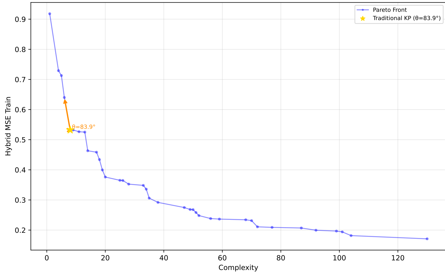
522_pm10 - Run 13 - SVP - Hybrid MSE Train \lambda_1=0.00, \lambda_2=0.10, \lambda_3=0.00 | Difficulty: 0.95 | Method: hmr
