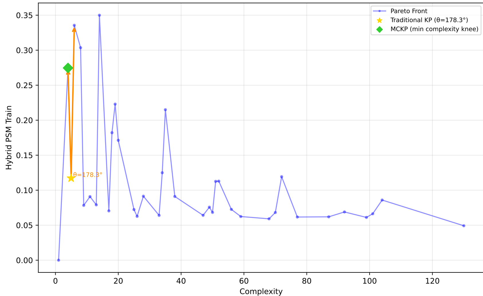
522_pm10 - Run 13 - SVP - Hybrid PSM Train \lambda_1=1.00, \lambda_2=0.00, \lambda_3=0.90 | Difficulty: 0.95 | Method: hmr
