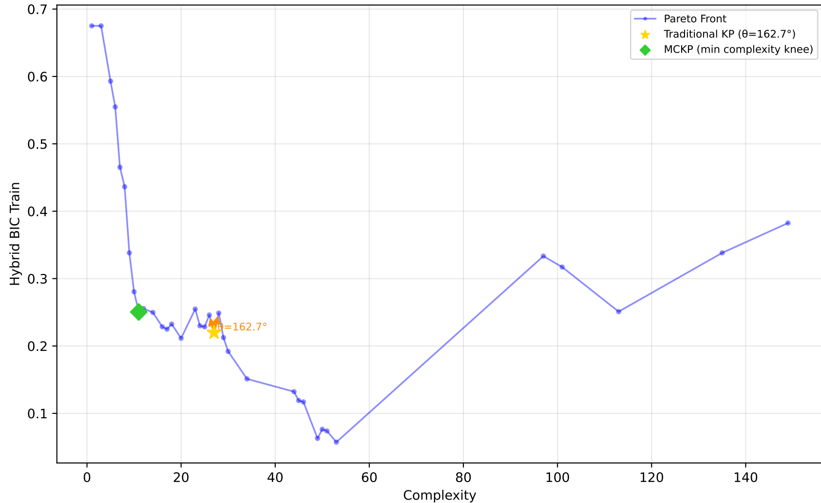
522_pm10 - Run 14 - MVP - Hybrid BIC Train \lambda_1=0.00, \lambda_2=0.90, \lambda_3=0.00 | Difficulty: 1.00 | Method: hmr
