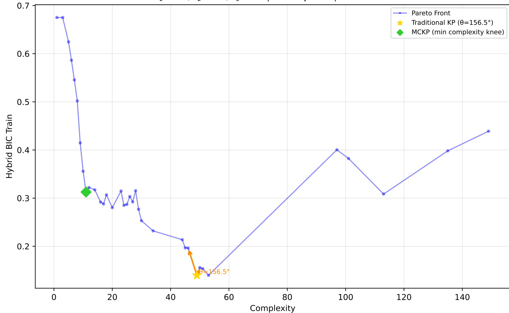
522_pm10 - Run 14 - MVP - Hybrid BIC Train \lambda_1=1.00, \lambda_2=0.00, \lambda_3=0.00 | Difficulty: 1.00 | Method: hmr
