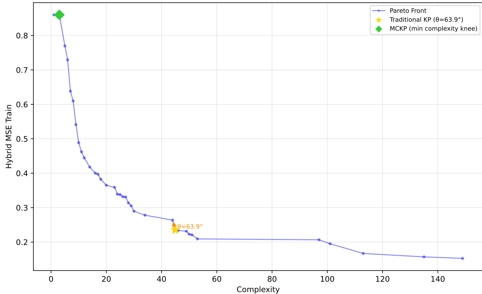
522_pm10 - Run 14 - MVP - Hybrid MSE Train \lambda_1=0.00, \lambda_2=0.90, \lambda_3=0.00 | Difficulty: 1.00 | Method: hmr
