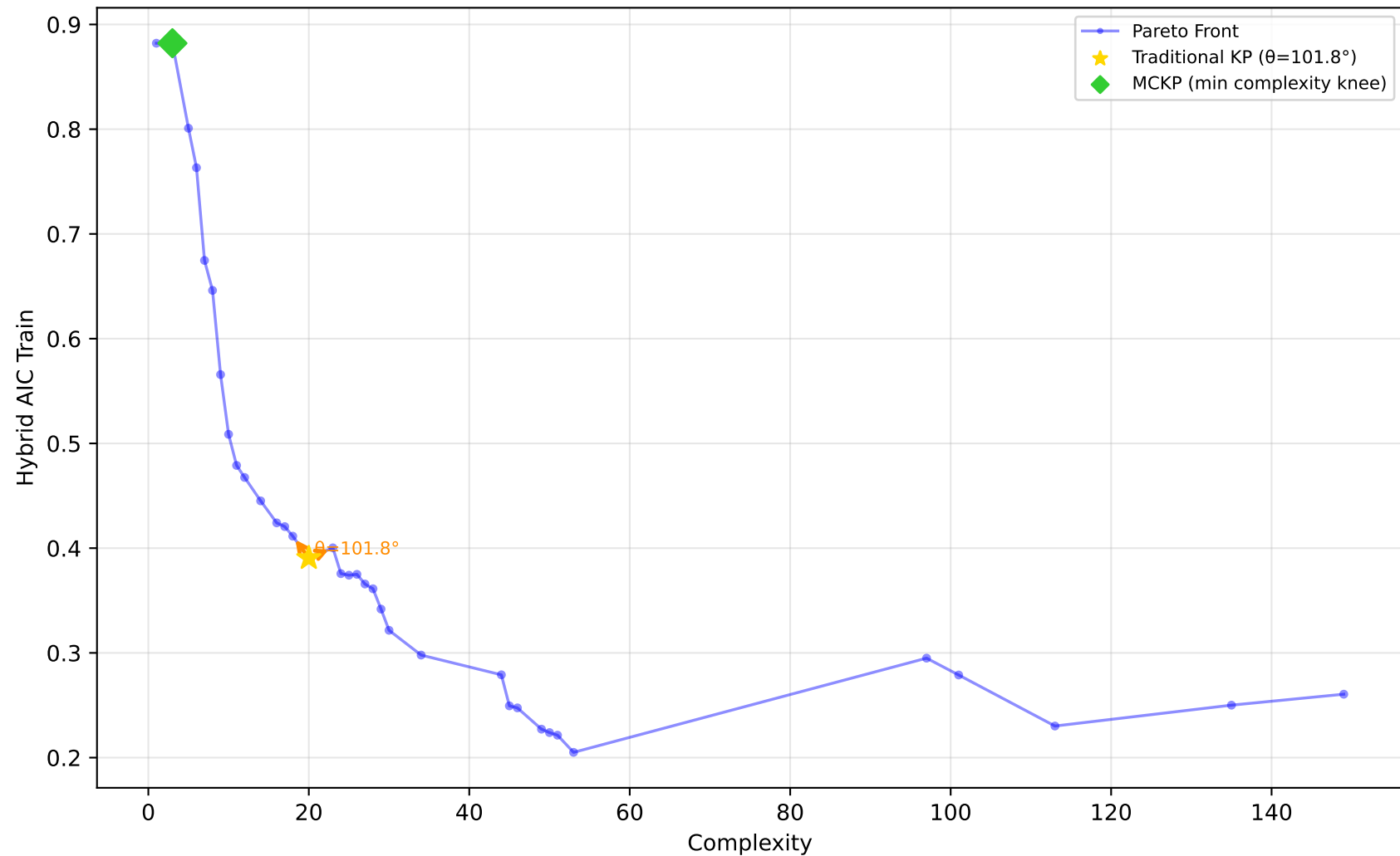
522_pm10 - Run 14 - SVP - Hybrid AIC Train \lambda_1=0.00, \lambda_2=0.10, \lambda_3=0.00 | Difficulty: 1.00 | Method: hmr
