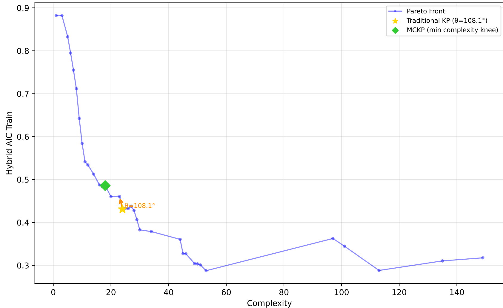
522_pm10 - Run 14 - SVP - Hybrid AIC Train \lambda_1=1.00, \lambda_2=0.00, \lambda_3=0.90 | Difficulty: 1.00 | Method: hmr
